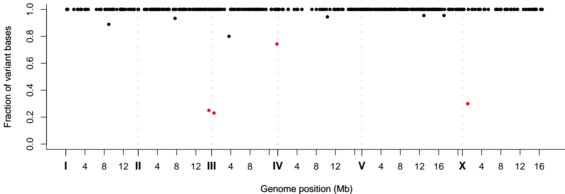
Fraction of Variant Bases at Position, Strain VC40254
