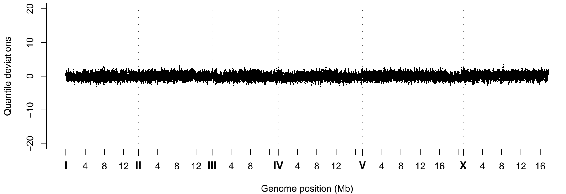
Quantile Deviations, Strain VC40254
