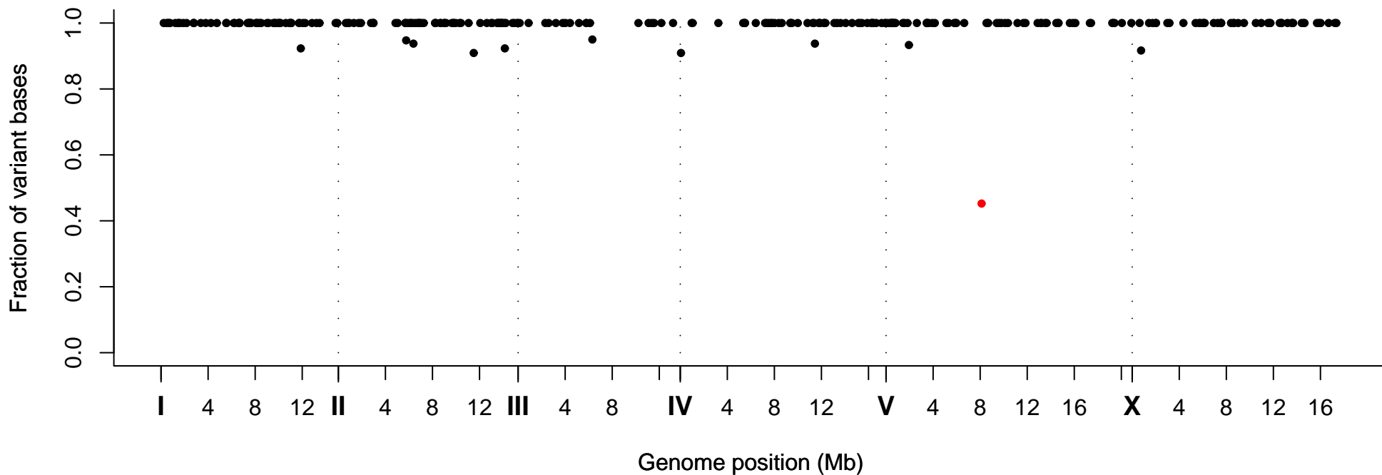
Fraction of Variant Bases at Position, Strain VC40255
