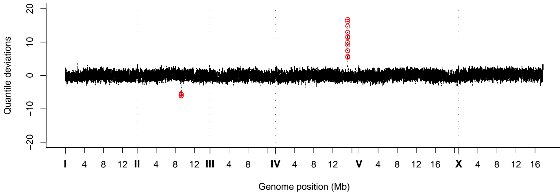
Quantile Deviations, Strain VC40255
