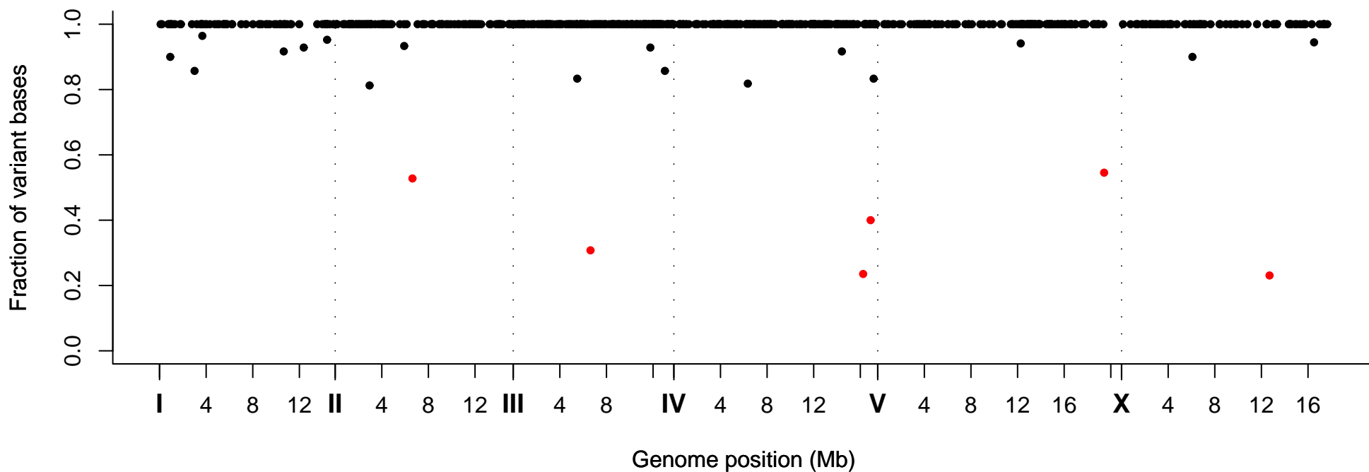
Fraction of Variant Bases at Position, Strain VC40257
