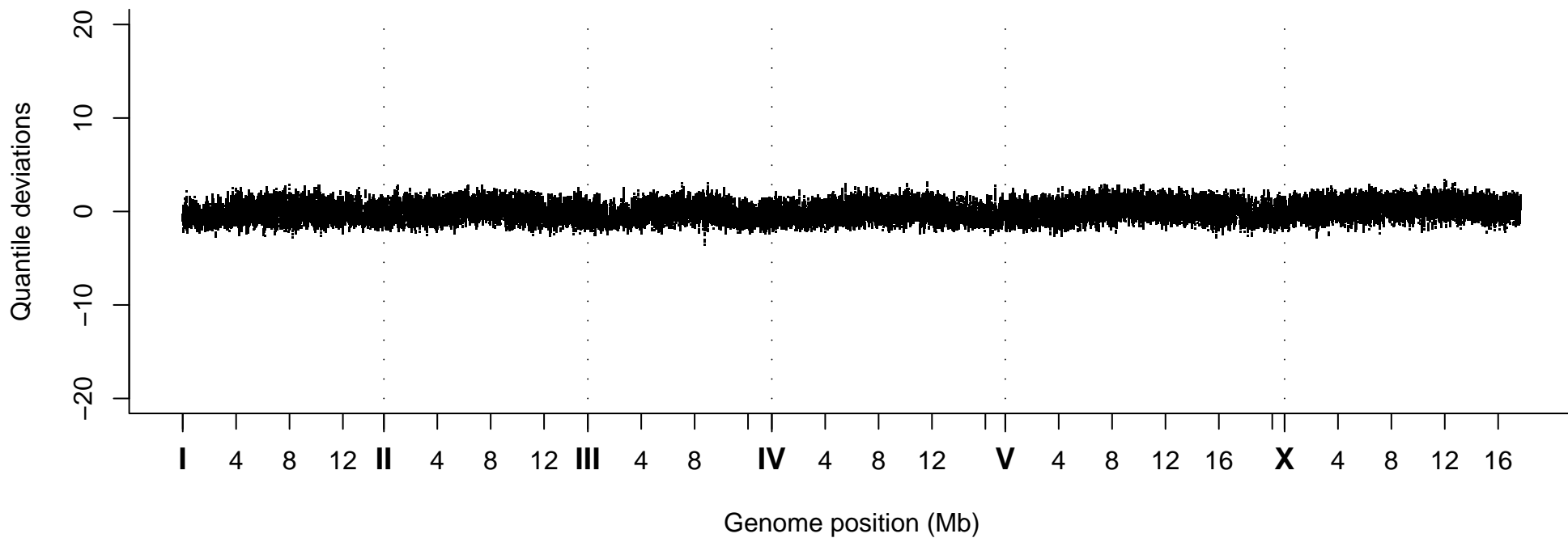
Quantile Deviations, Strain VC40257
