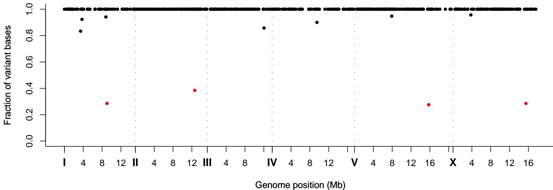
Fraction of Variant Bases at Position, Strain VC40259
