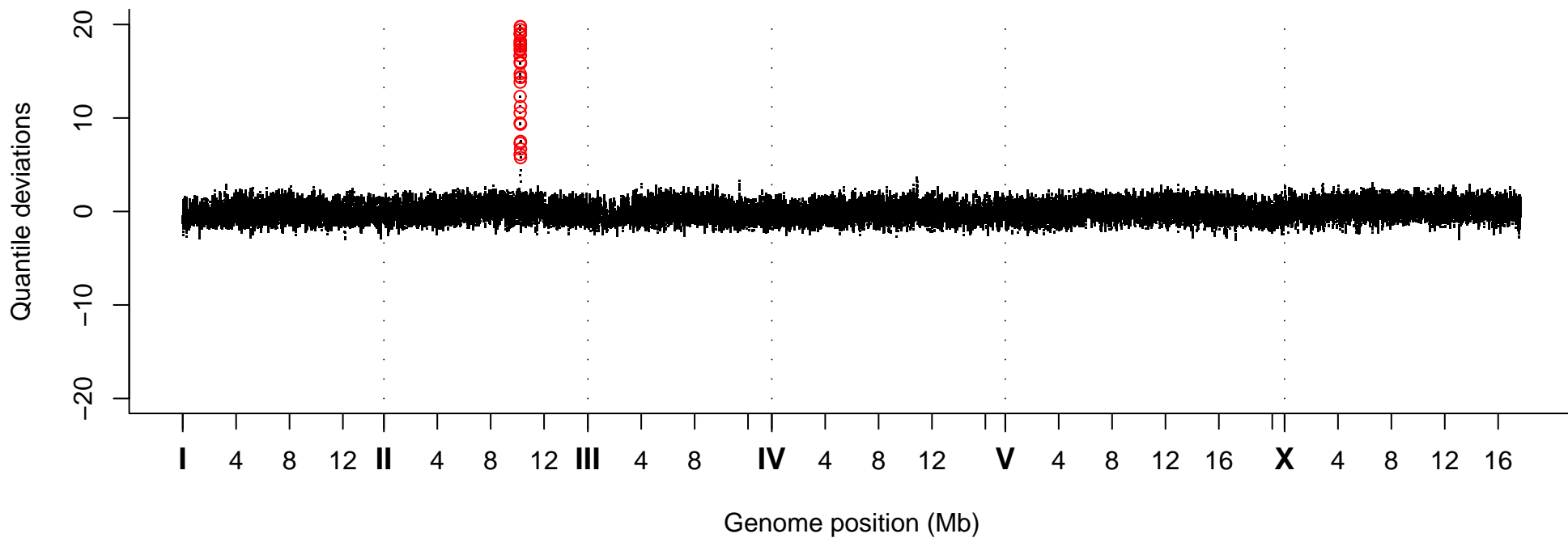
Quantile Deviations, Strain VC40259
