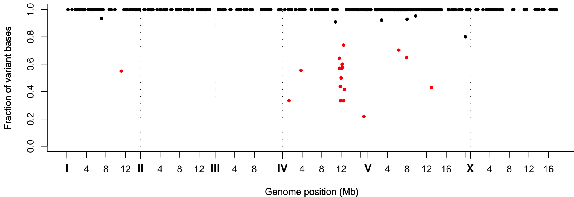
Fraction of Variant Bases at Position, Strain VC40260
