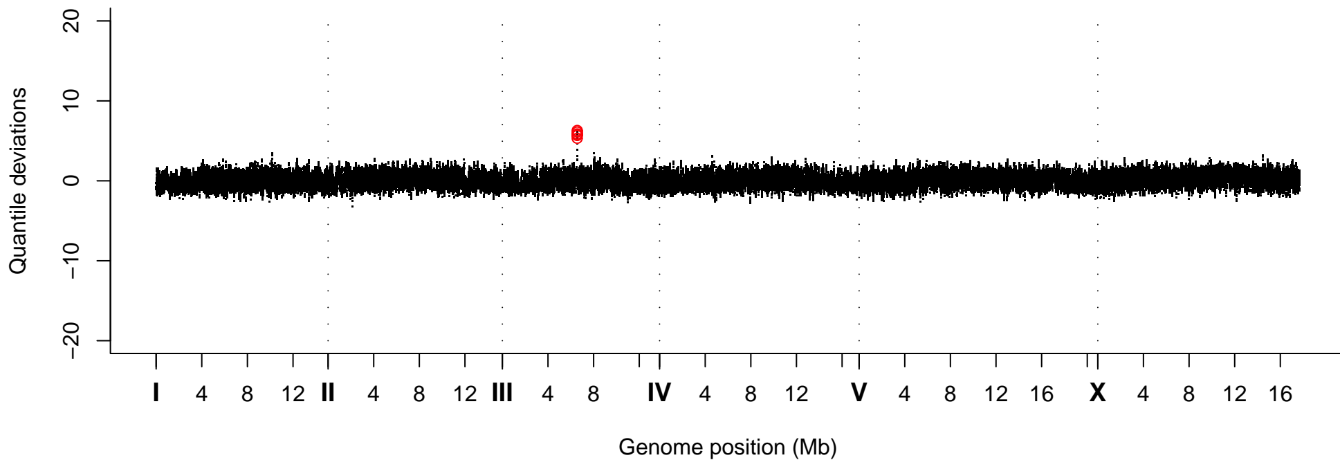
Quantile Deviations, Strain VC40260
