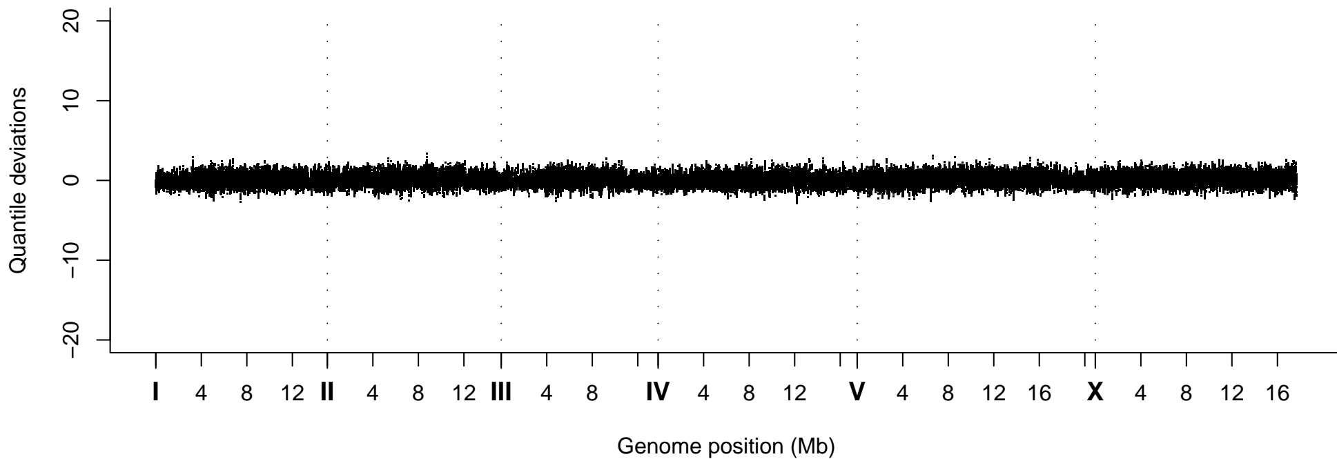
Quantile Deviations, Strain VC40261
