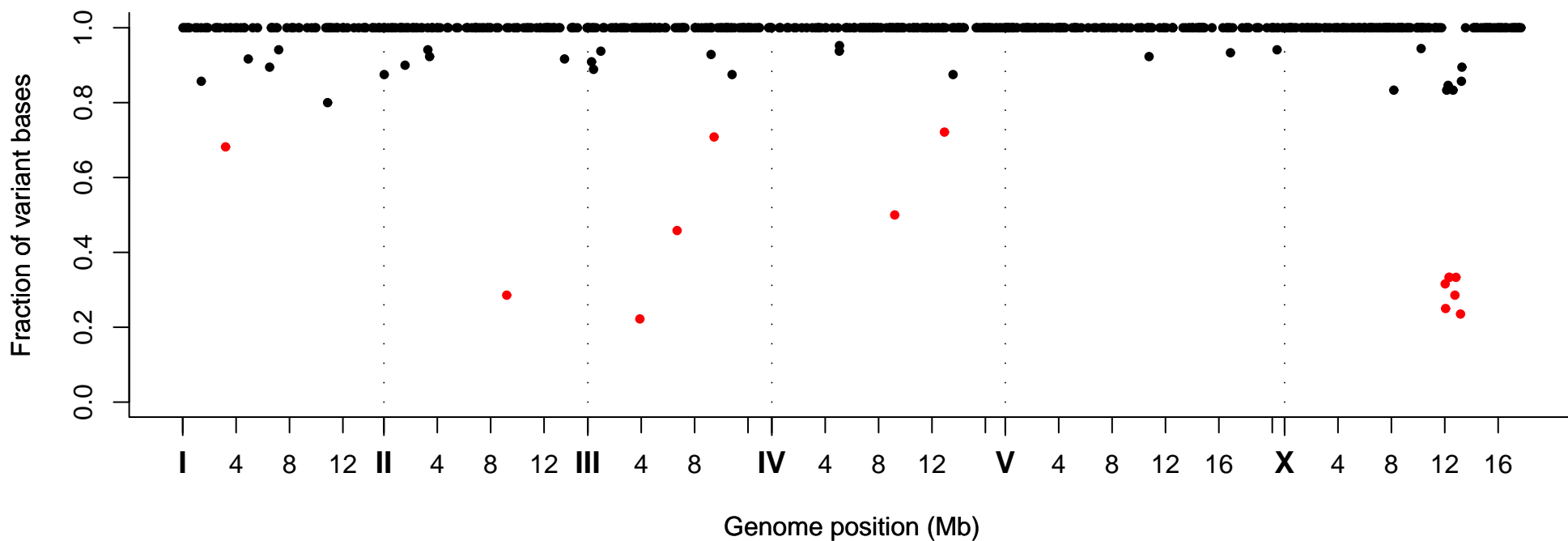
Fraction of Variant Bases at Position, Strain VC40261
