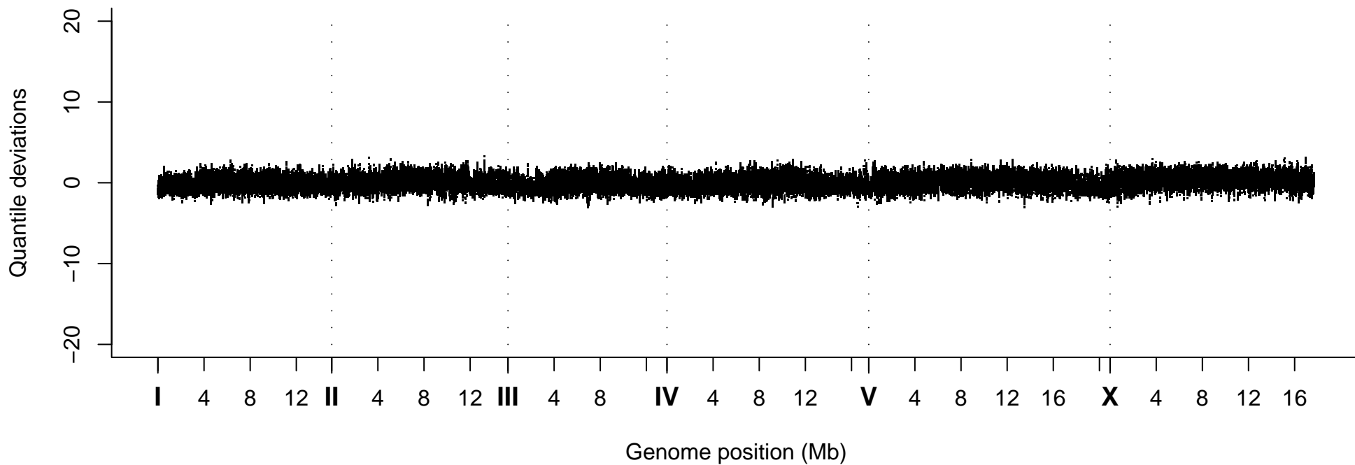
Quantile Deviations, Strain VC40262
