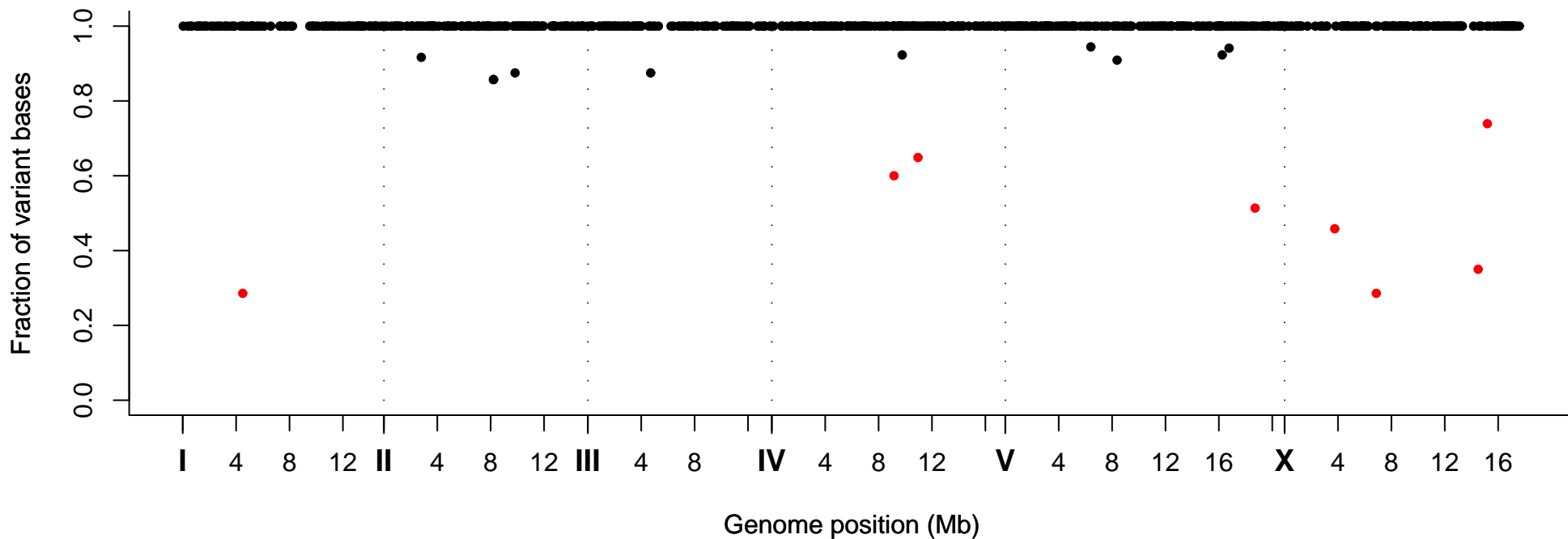
Fraction of Variant Bases at Position, Strain VC40262
