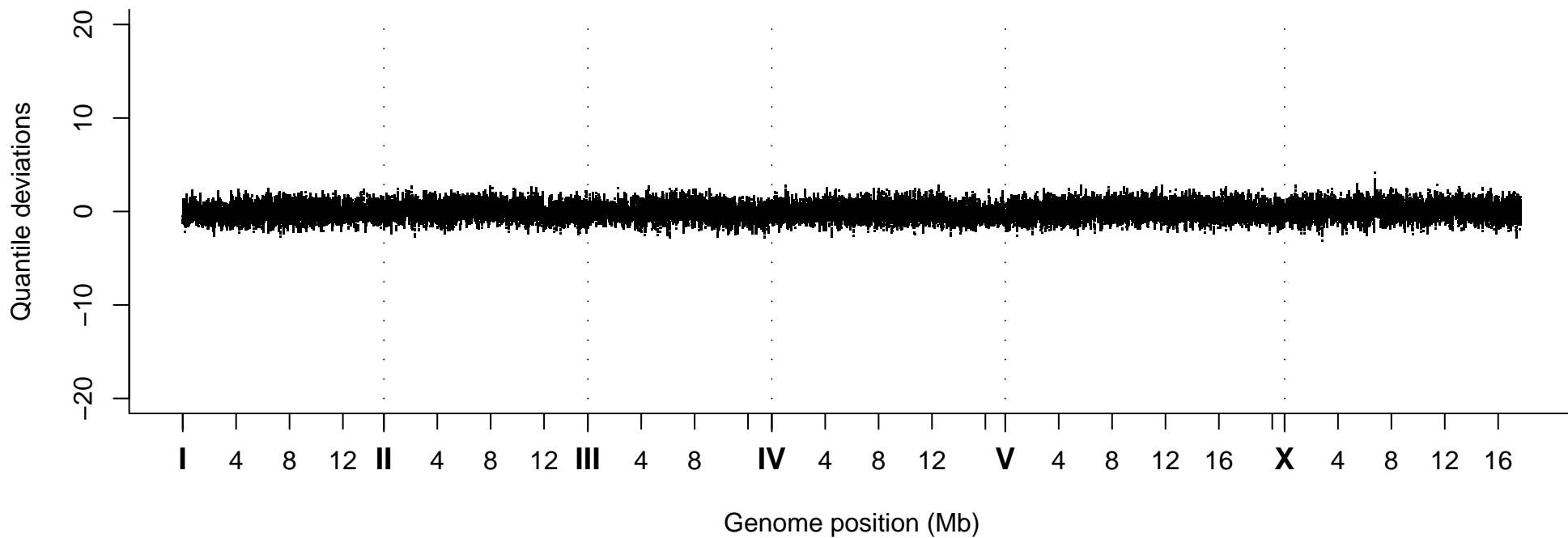
Quantile Deviations, Strain VC40266
