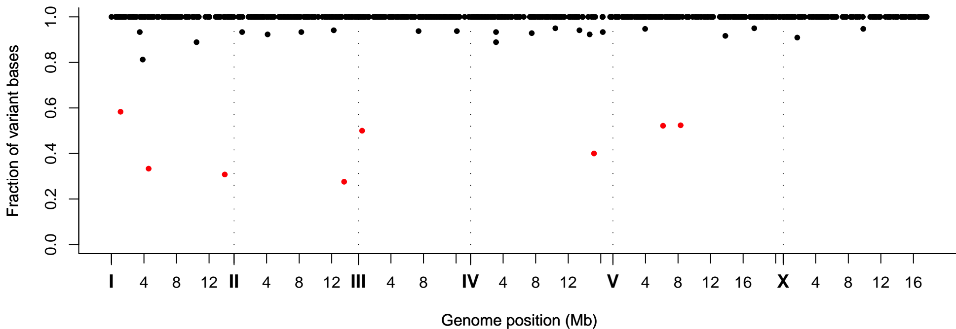
Fraction of Variant Bases at Position, Strain VC40266
