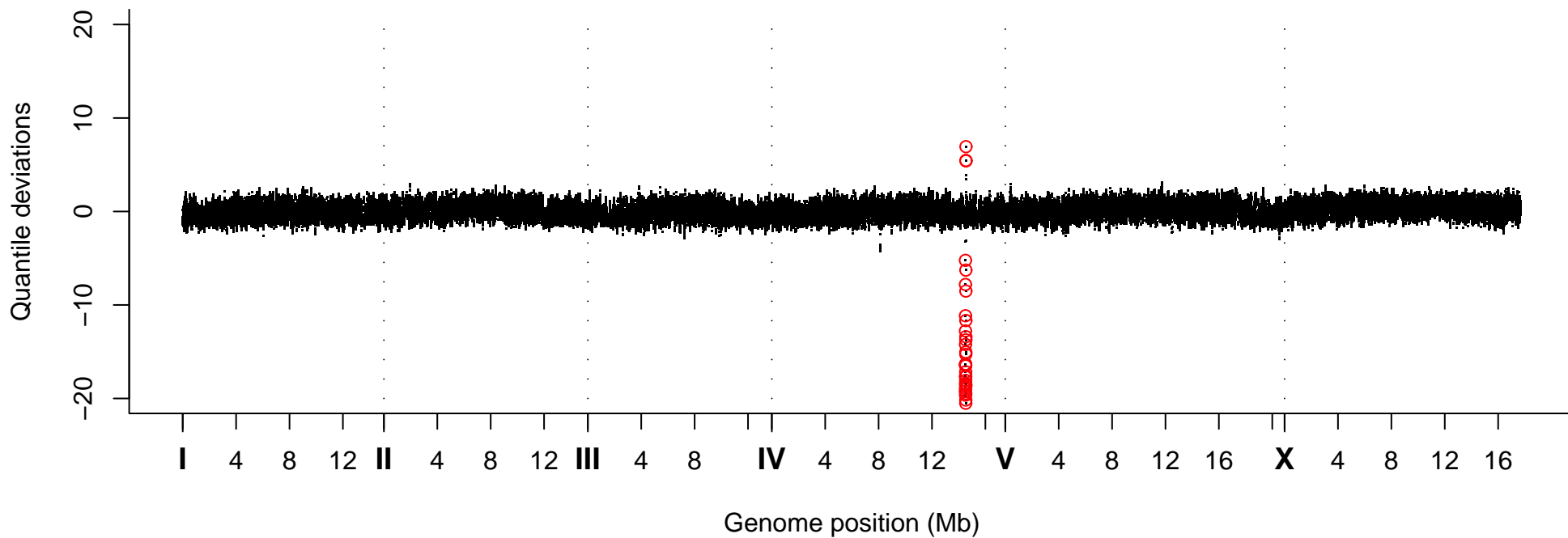
Quantile Deviations, Strain VC40268
