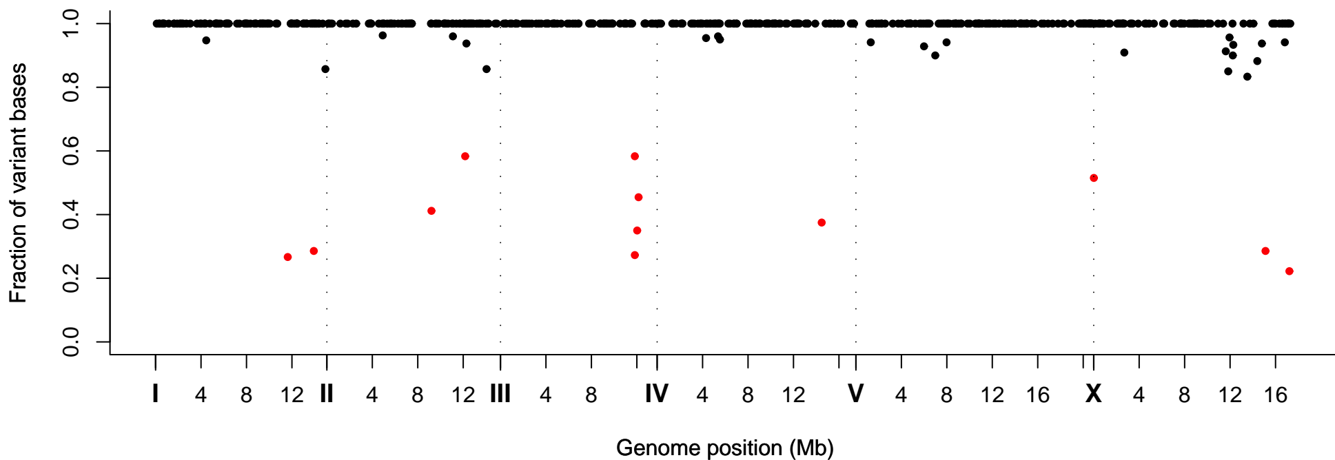
Fraction of Variant Bases at Position, Strain VC40268
