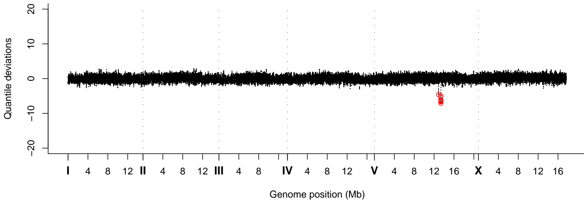
Quantile Deviations, Strain VC40273
