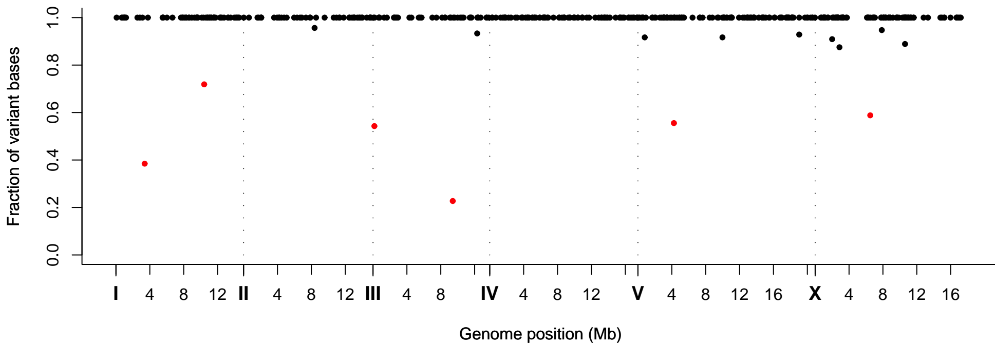
Fraction of Variant Bases at Position, Strain VC40273
