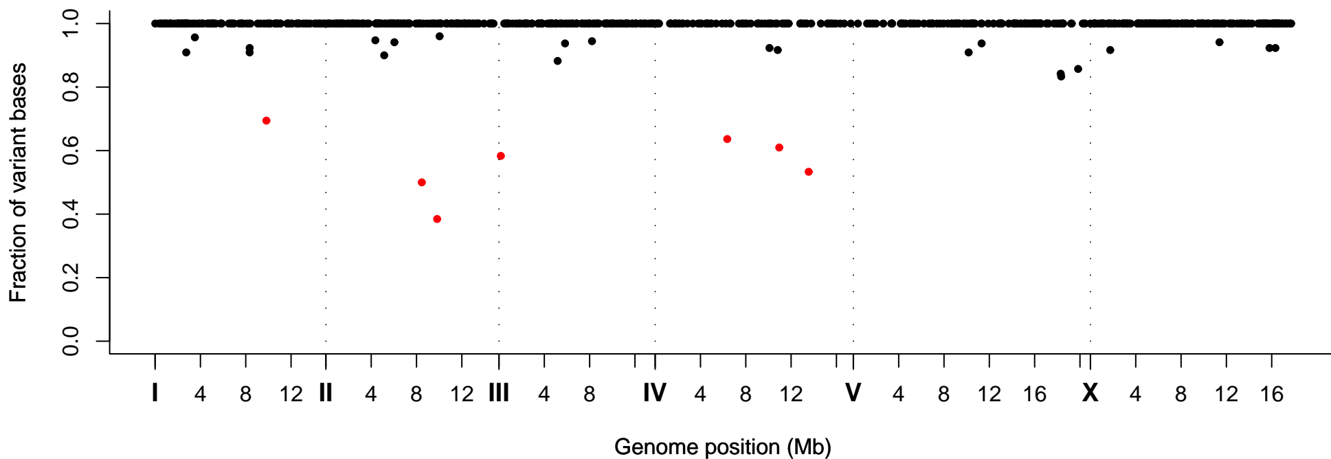
Fraction of Variant Bases at Position, Strain VC40274
