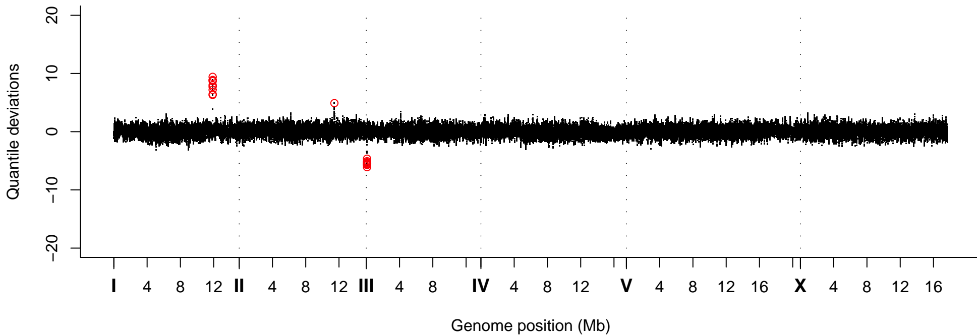
Quantile Deviations, Strain VC40274
