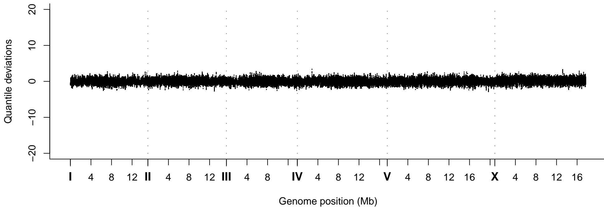
Quantile Deviations, Strain VC40282
