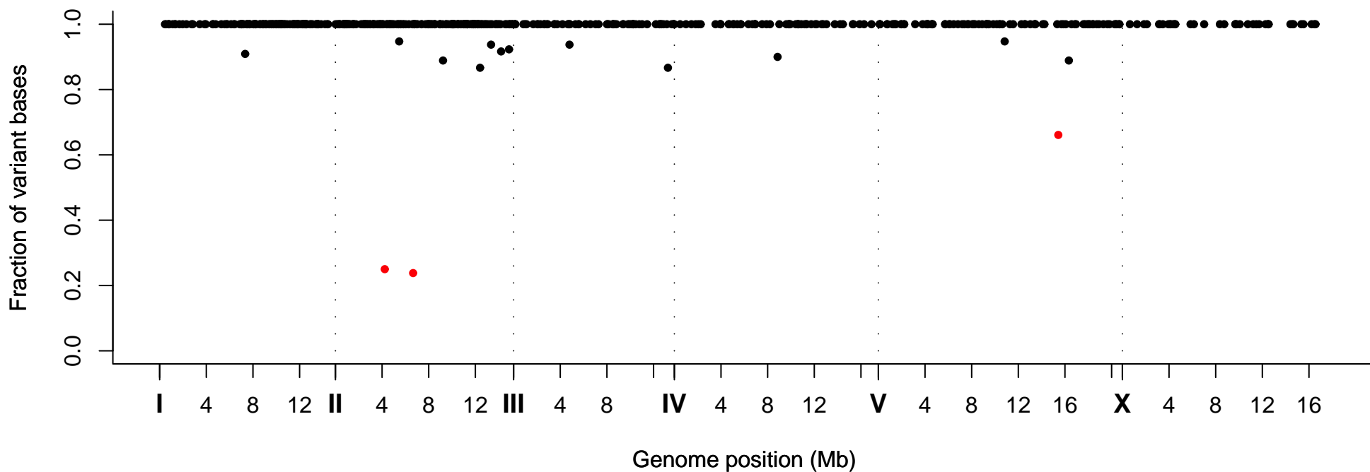
Fraction of Variant Bases at Position, Strain VC40282
