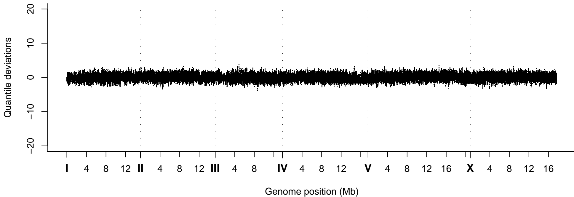
Quantile Deviations, Strain VC40284
