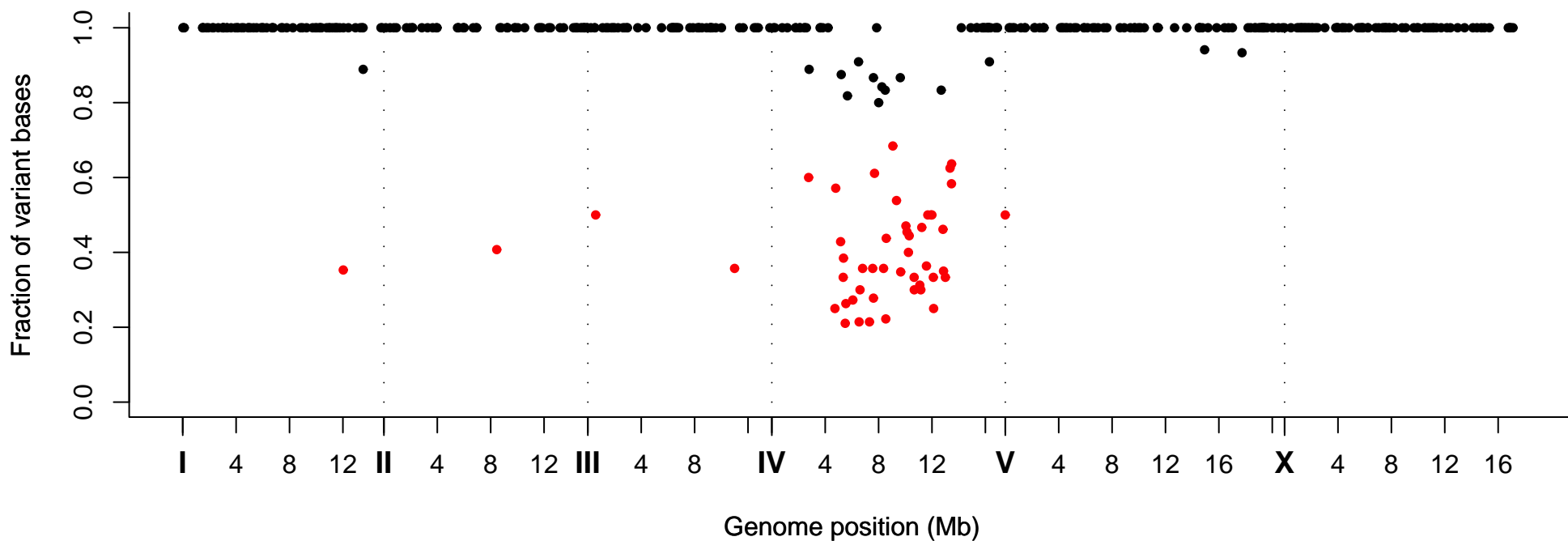
Fraction of Variant Bases at Position, Strain VC40284
