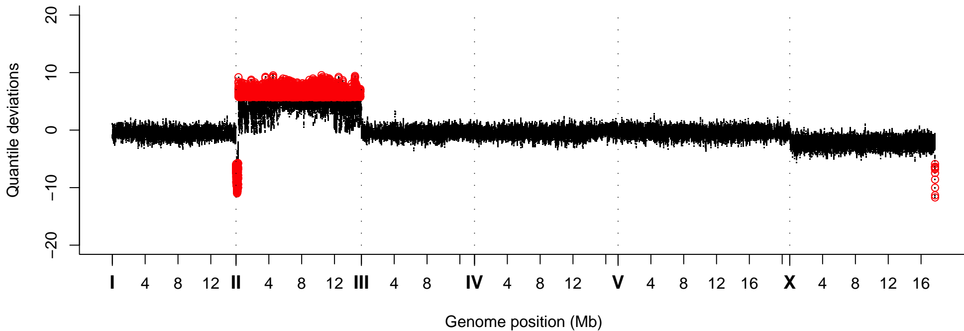
Quantile Deviations, Strain VC40287
