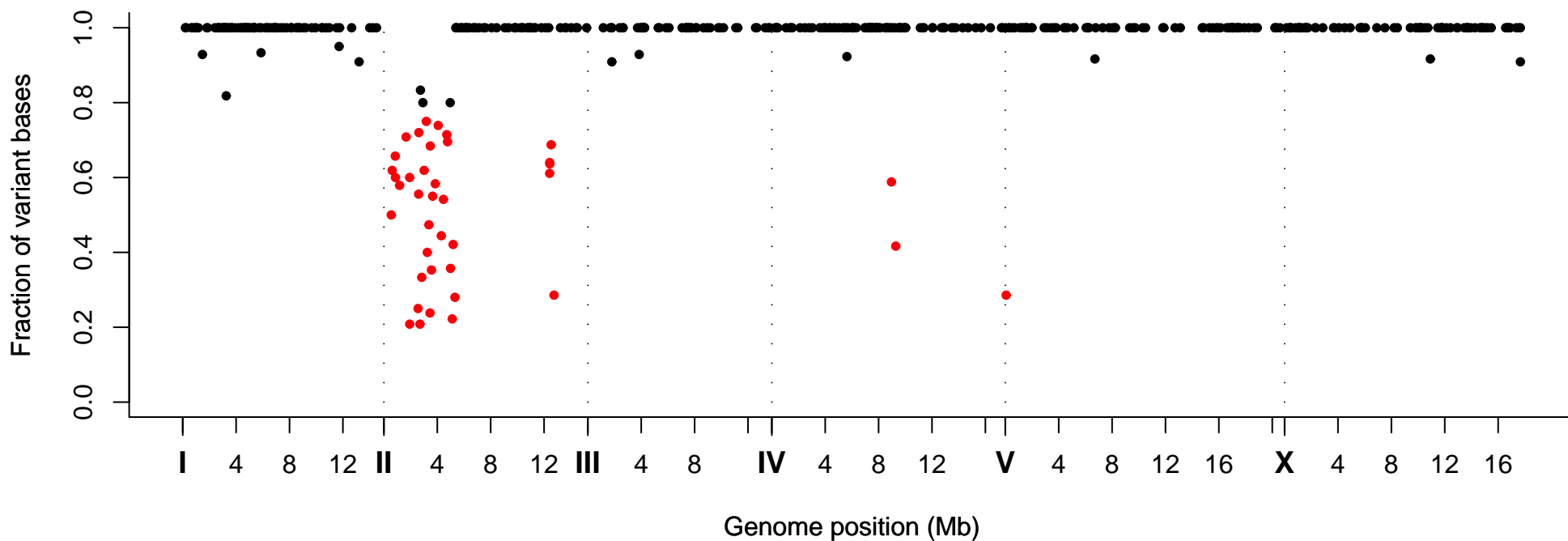
Fraction of Variant Bases at Position, Strain VC40287
