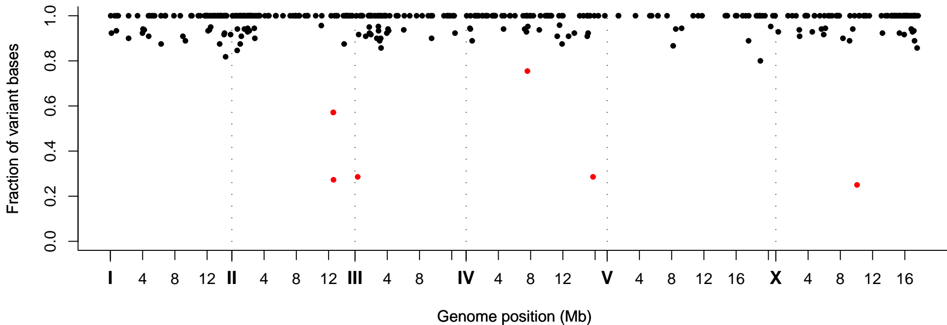
Fraction of Variant Bases at Position, Strain VC40289
