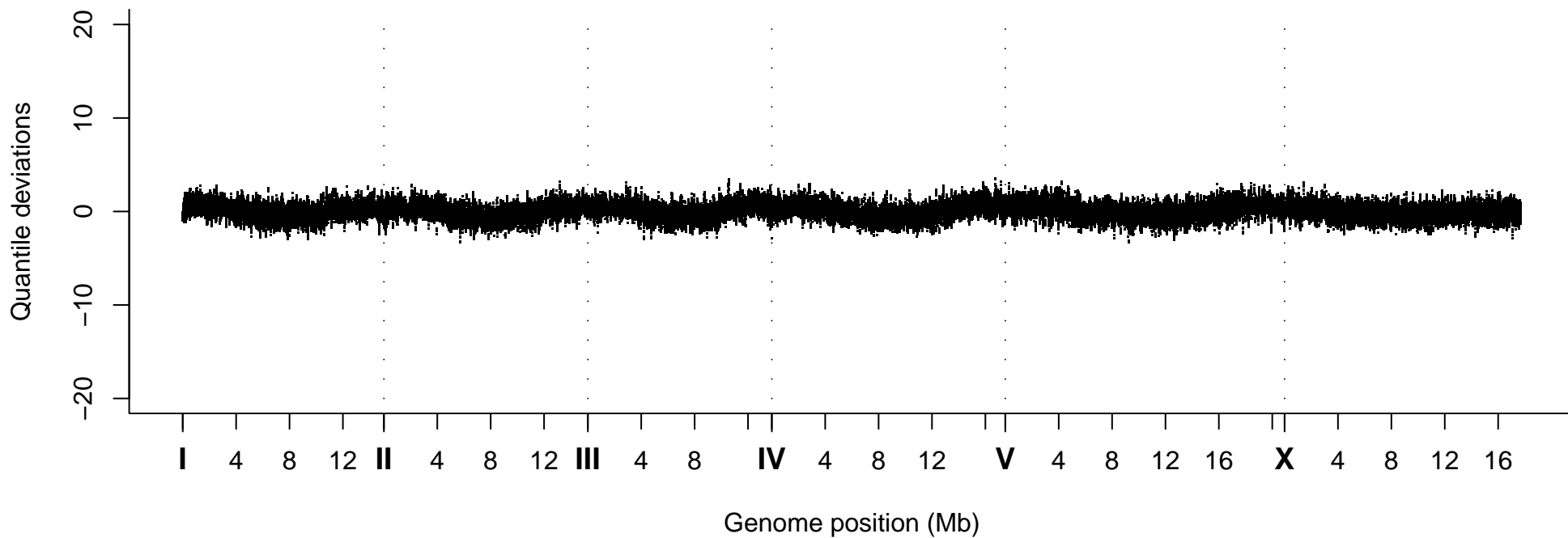
Quantile Deviations, Strain VC40289
