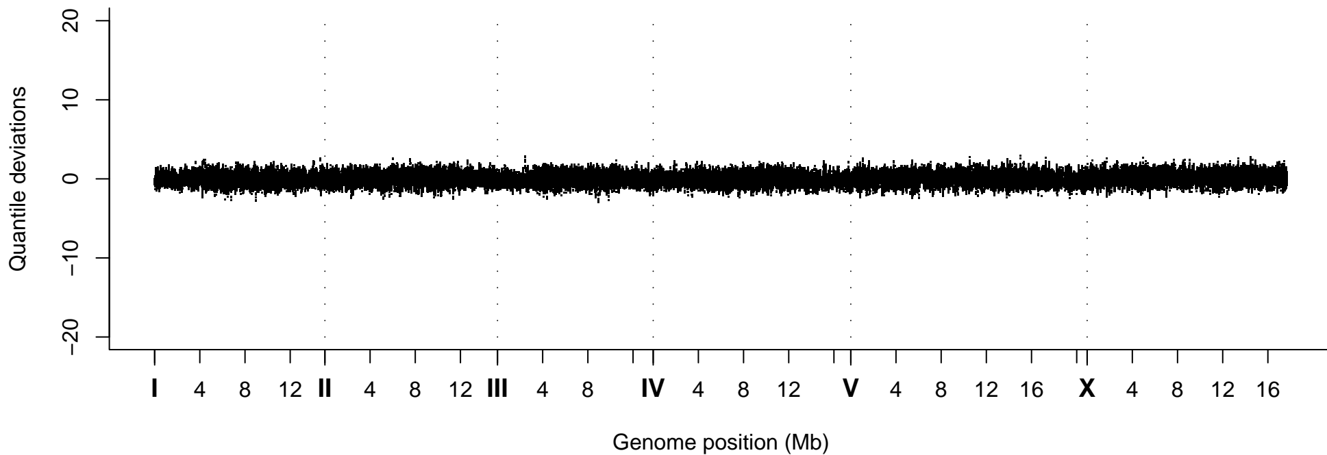
Quantile Deviations, Strain VC40296
