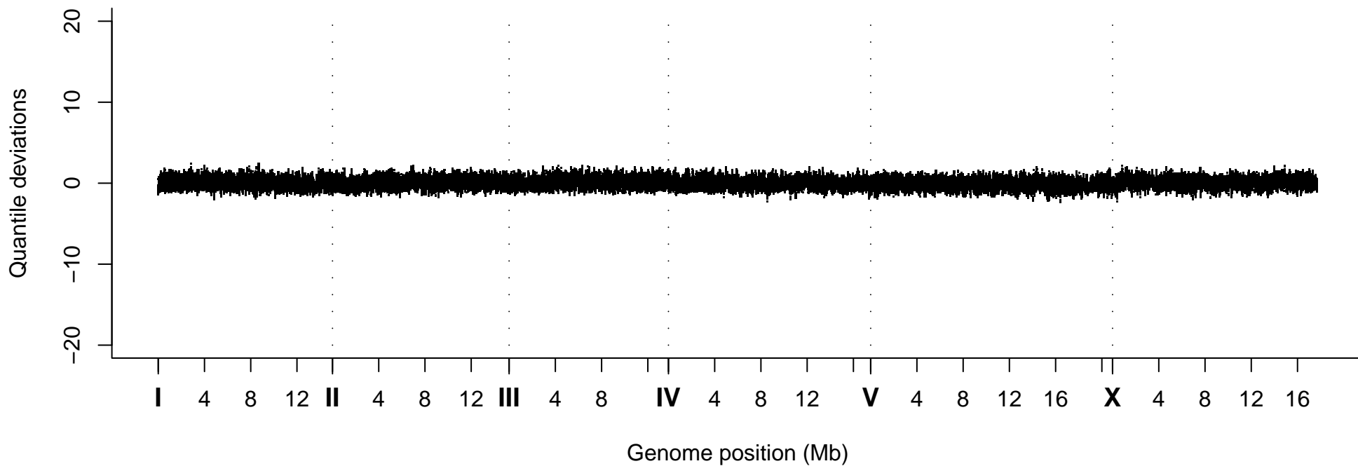
Quantile Deviations, Strain VC40297
