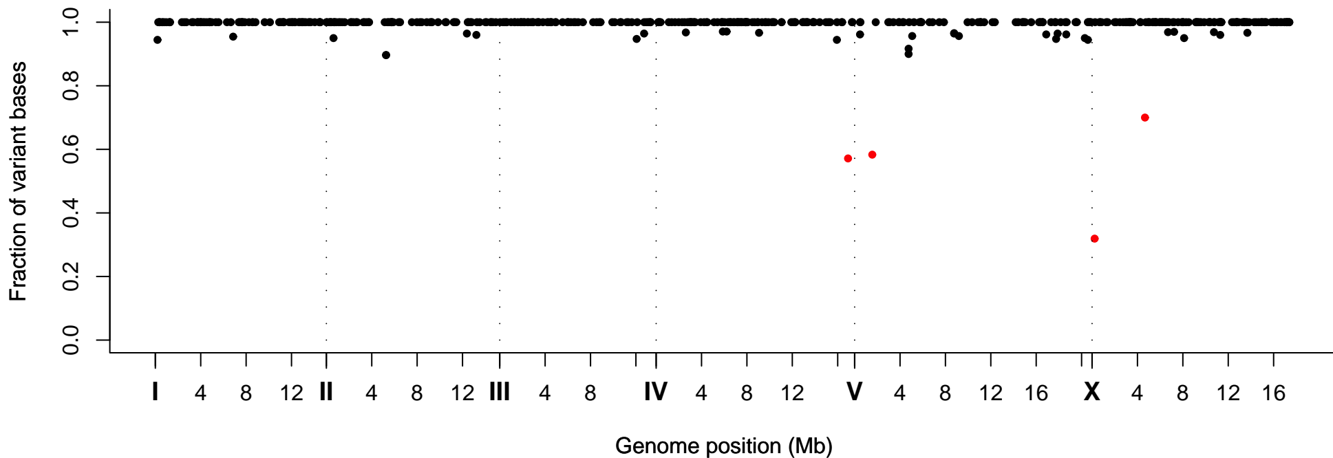
Fraction of Variant Bases at Position, Strain VC40297
