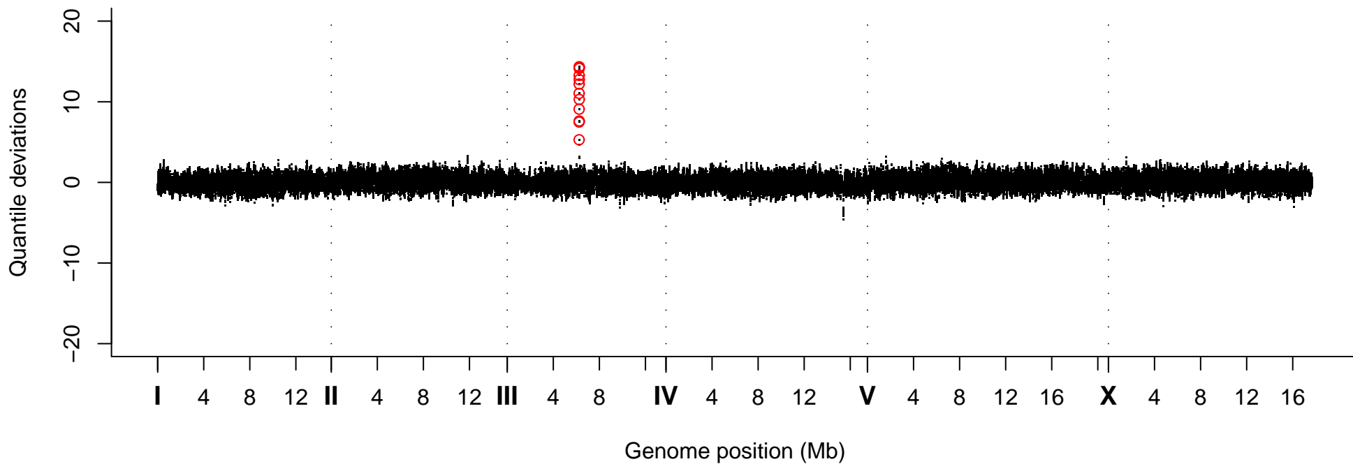
Quantile Deviations, Strain VC40300
