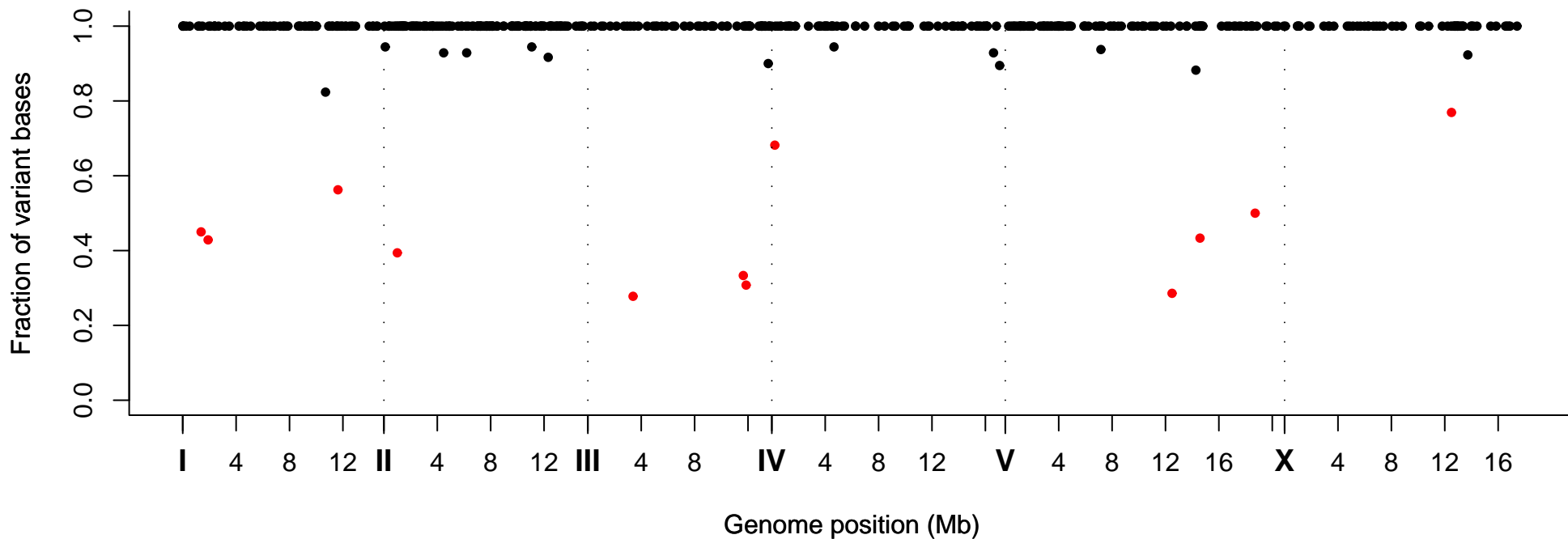
Fraction of Variant Bases at Position, Strain VC40300
