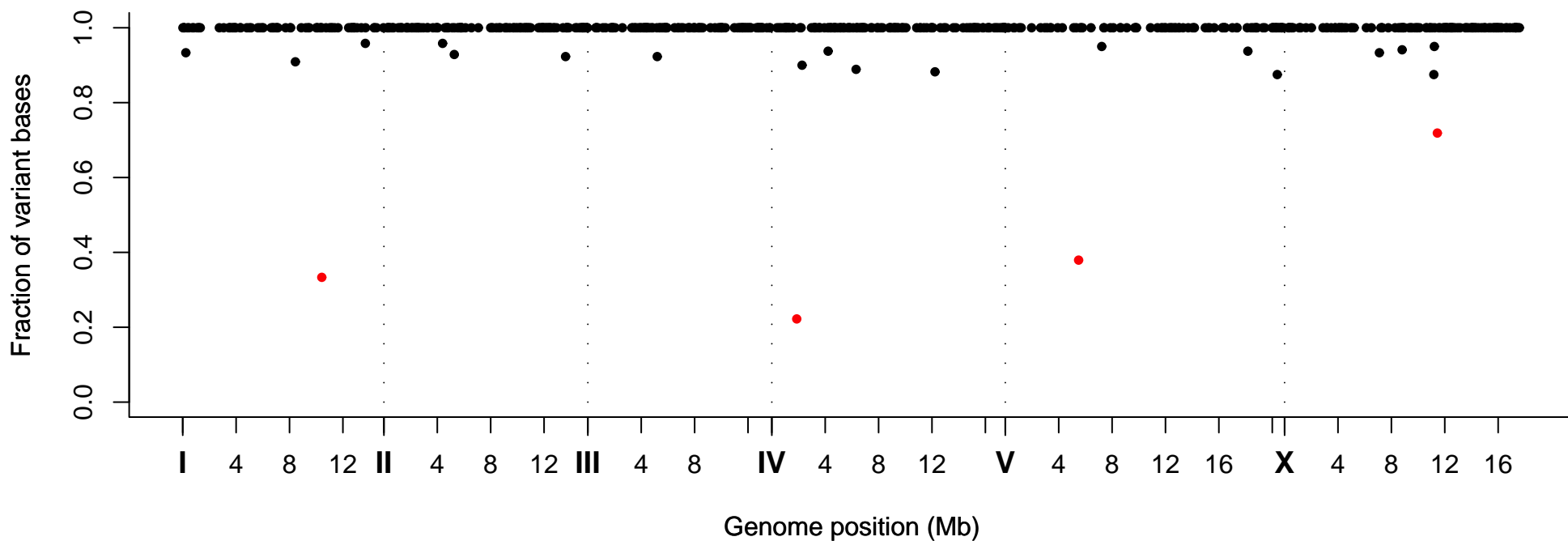
Fraction of Variant Bases at Position, Strain VC40304
