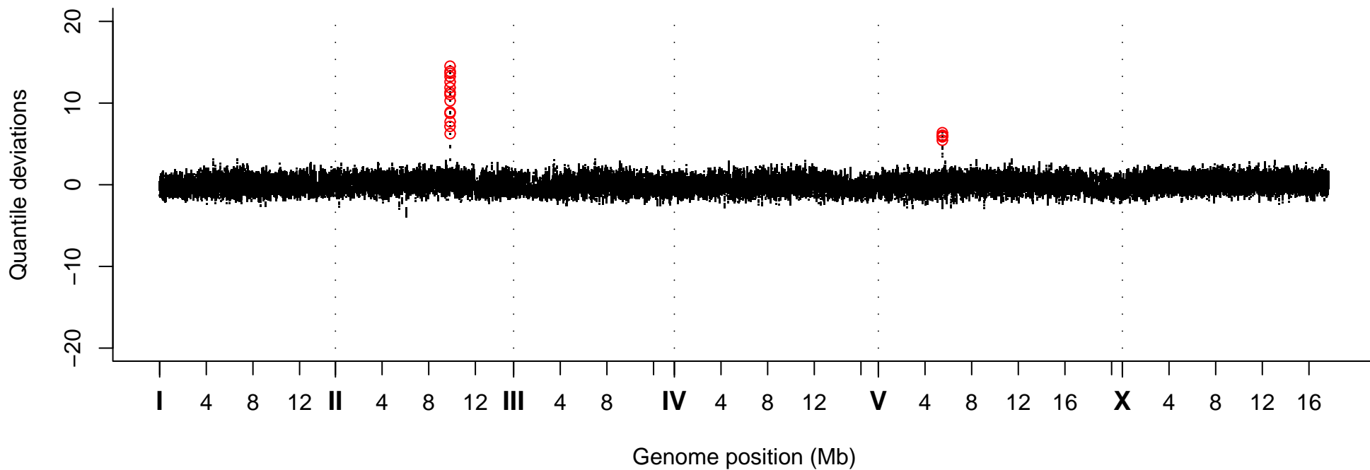
Quantile Deviations, Strain VC40304
