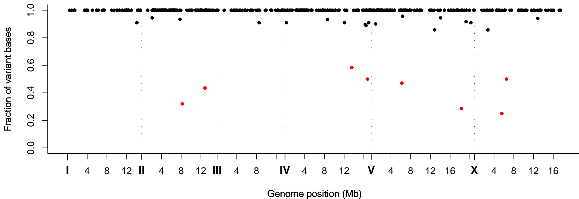
Fraction of Variant Bases at Position, Strain VC40310
