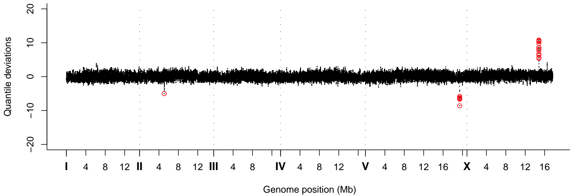
Quantile Deviations, Strain VC40310
