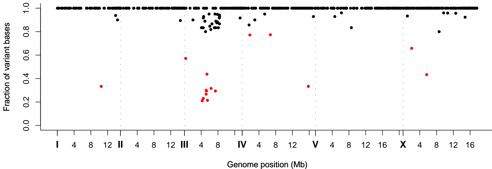
Fraction of Variant Bases at Position, Strain VC40315
