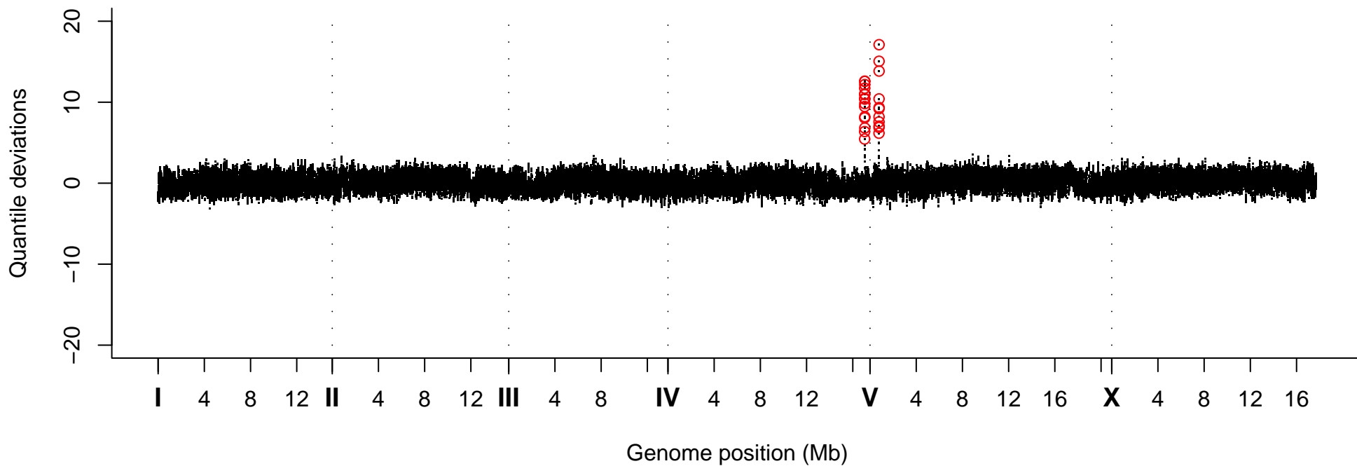
Quantile Deviations, Strain VC40315
