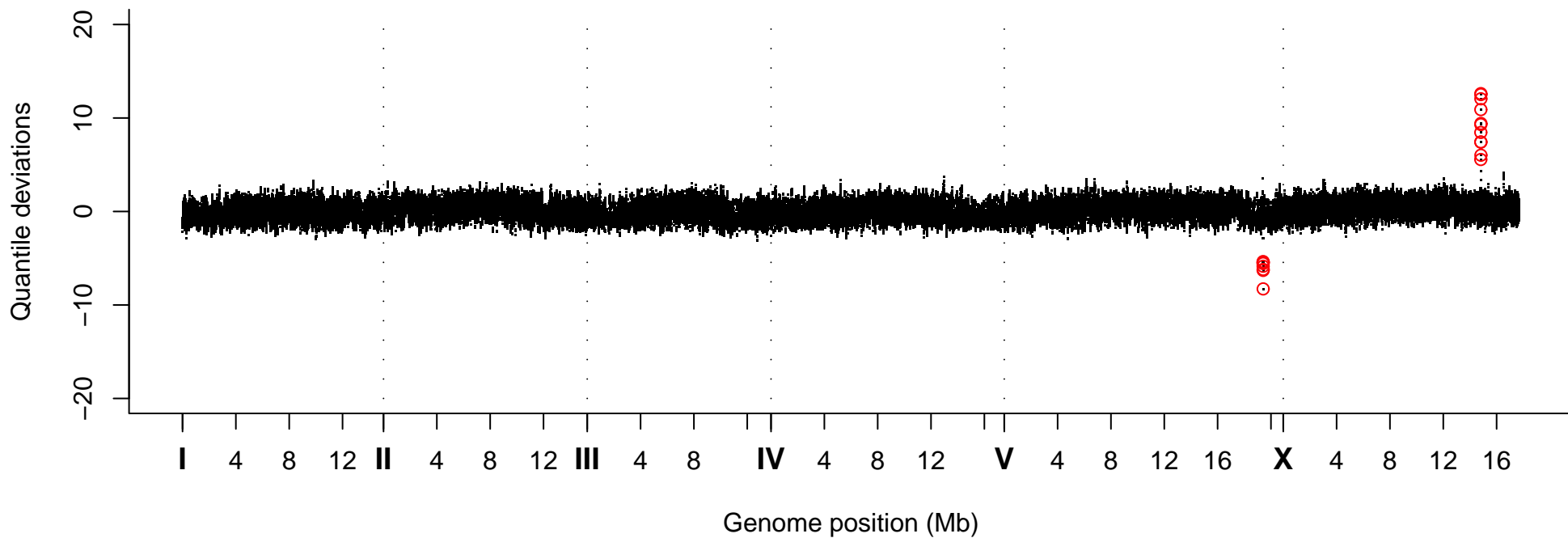
Quantile Deviations, Strain VC40317
