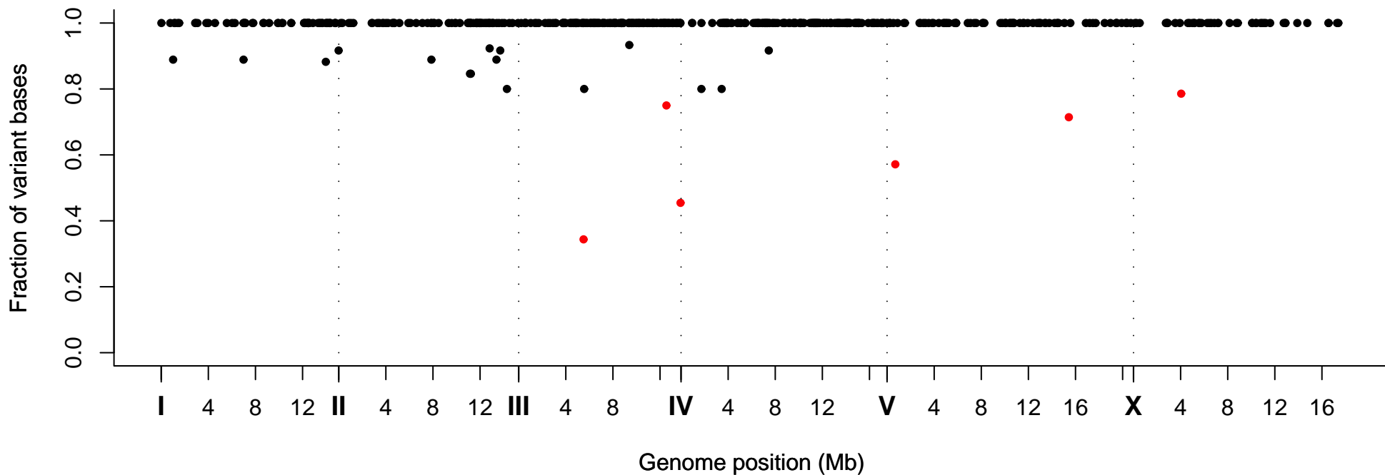
Fraction of Variant Bases at Position, Strain VC40317
