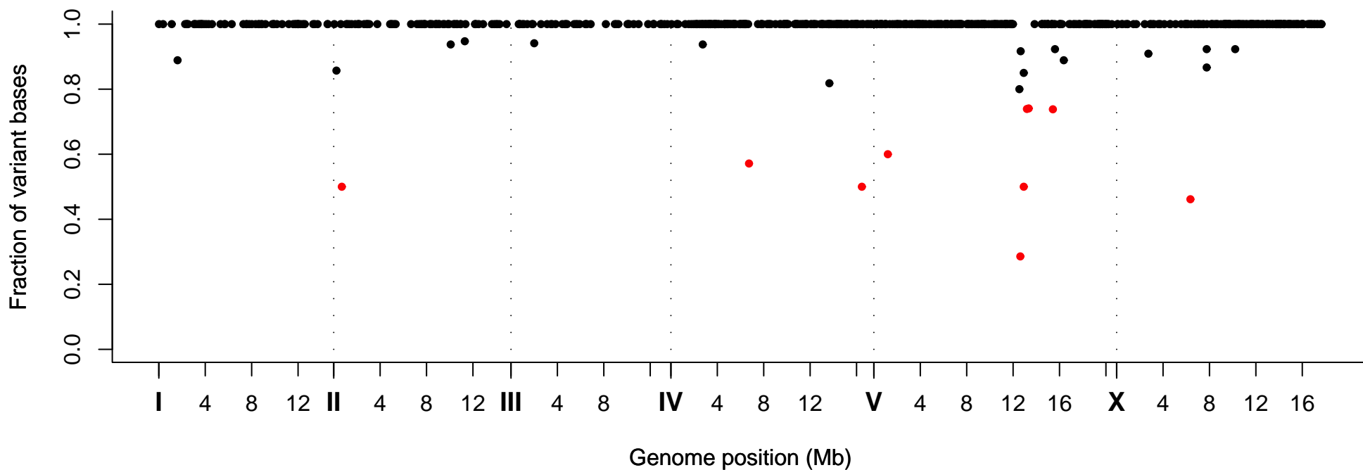
Fraction of Variant Bases at Position, Strain VC40320
