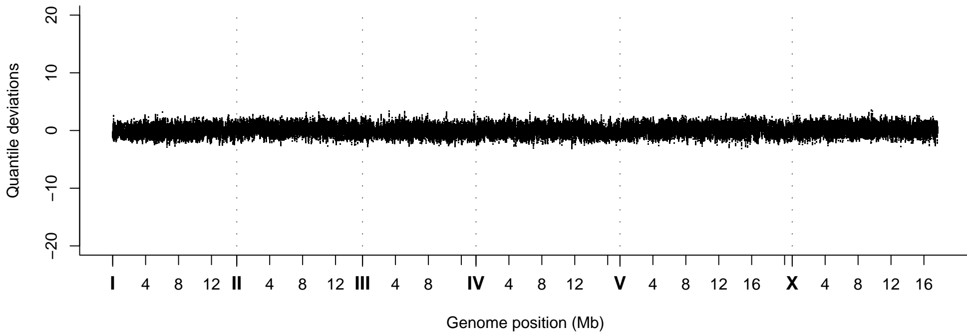
Quantile Deviations, Strain VC40320
