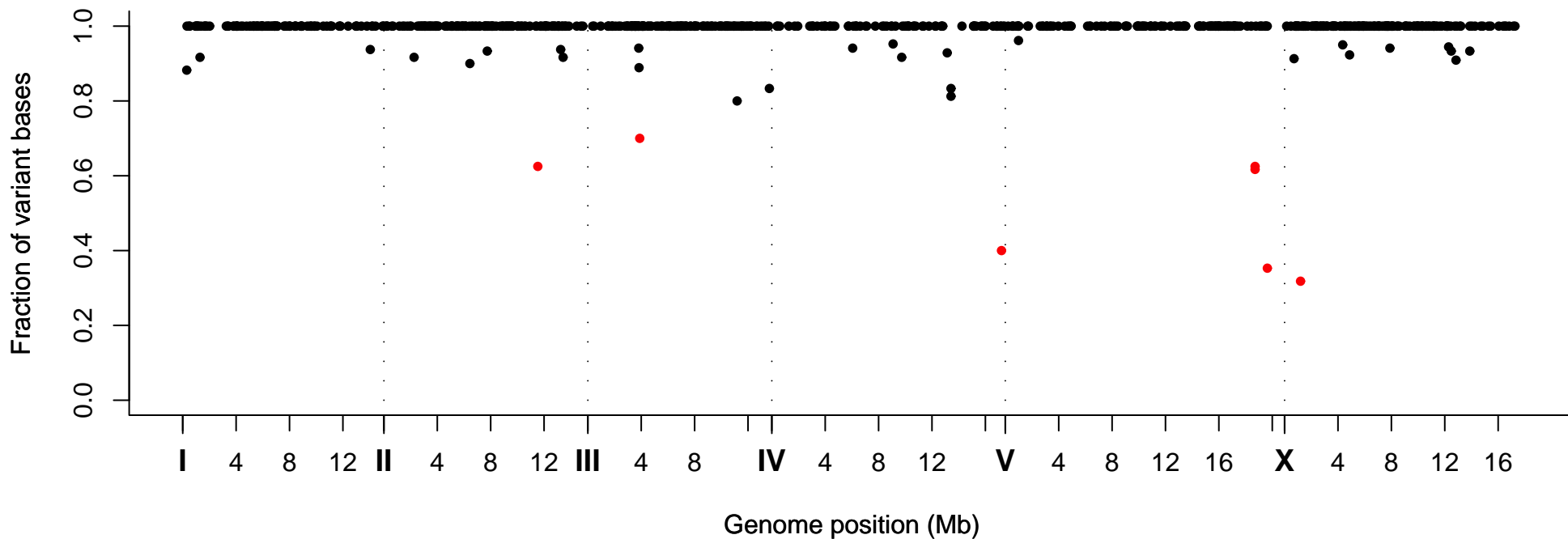
Fraction of Variant Bases at Position, Strain VC40321
