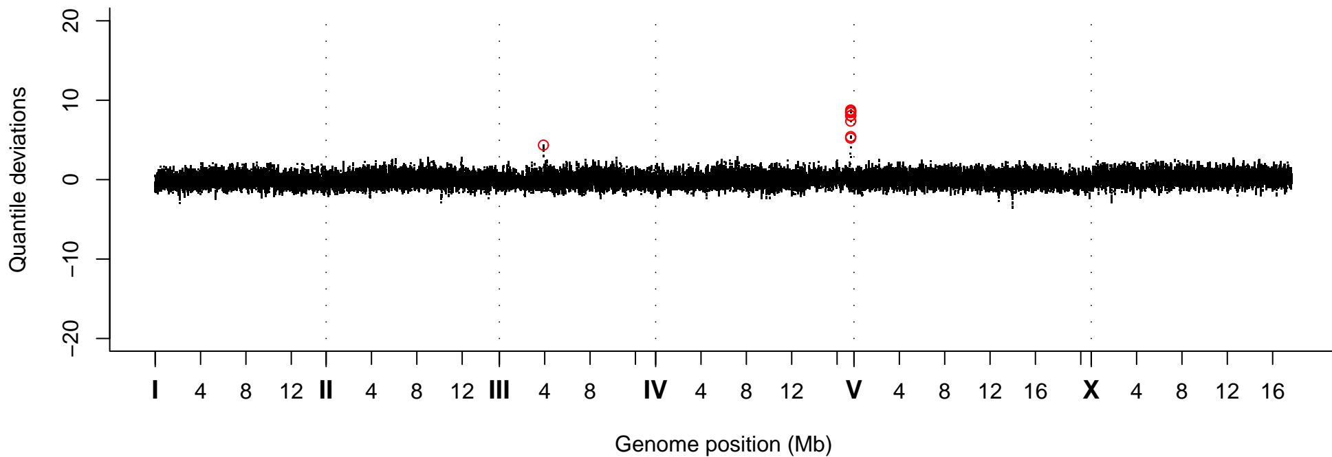
Quantile Deviations, Strain VC40321
