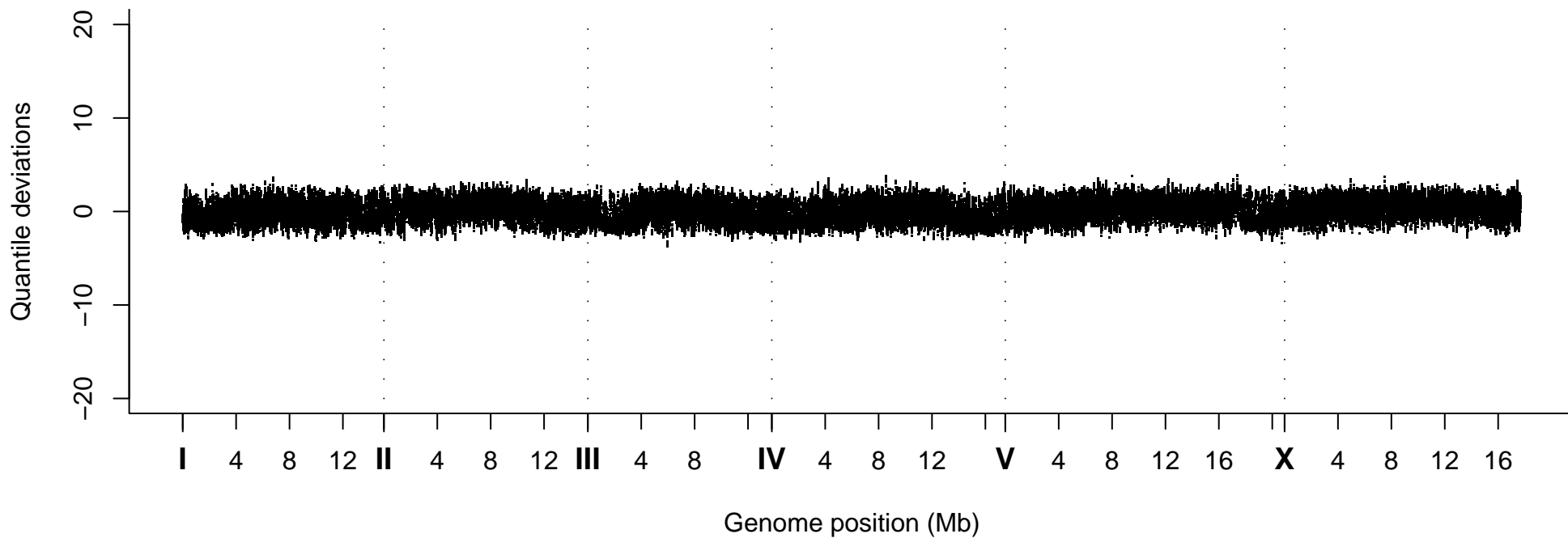
Quantile Deviations, Strain VC40322
