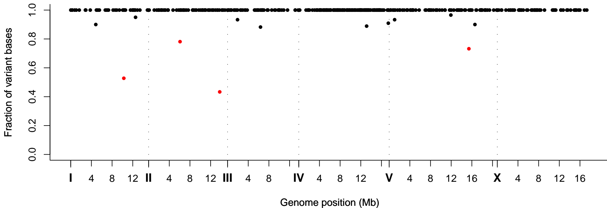
Fraction of Variant Bases at Position, Strain VC40322
