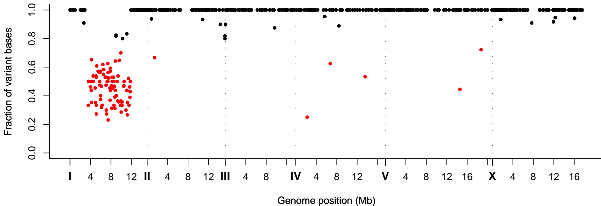
Fraction of Variant Bases at Position, Strain VC40327
