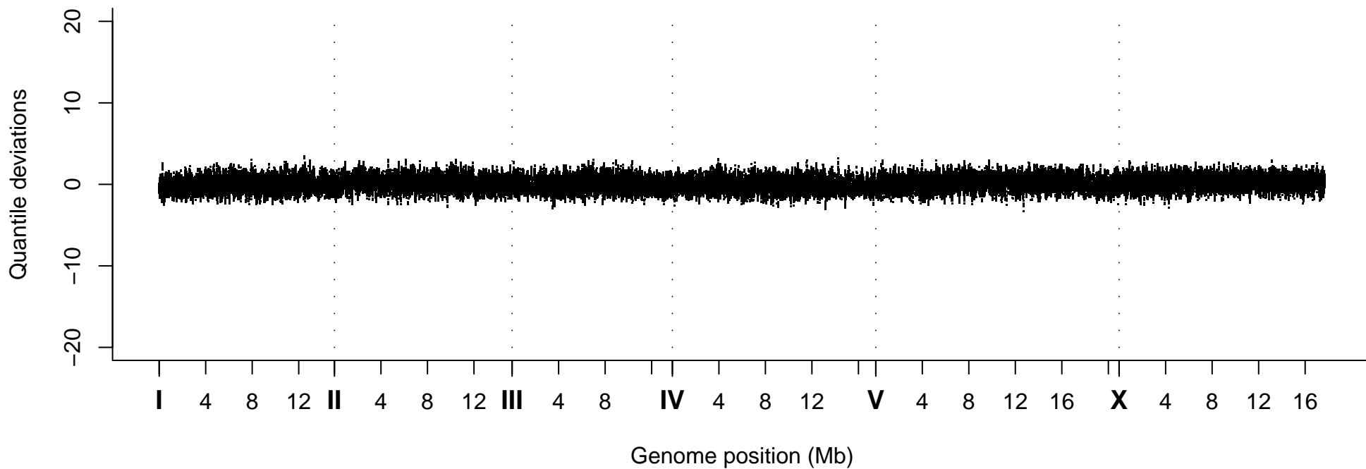
Quantile Deviations, Strain VC40327
