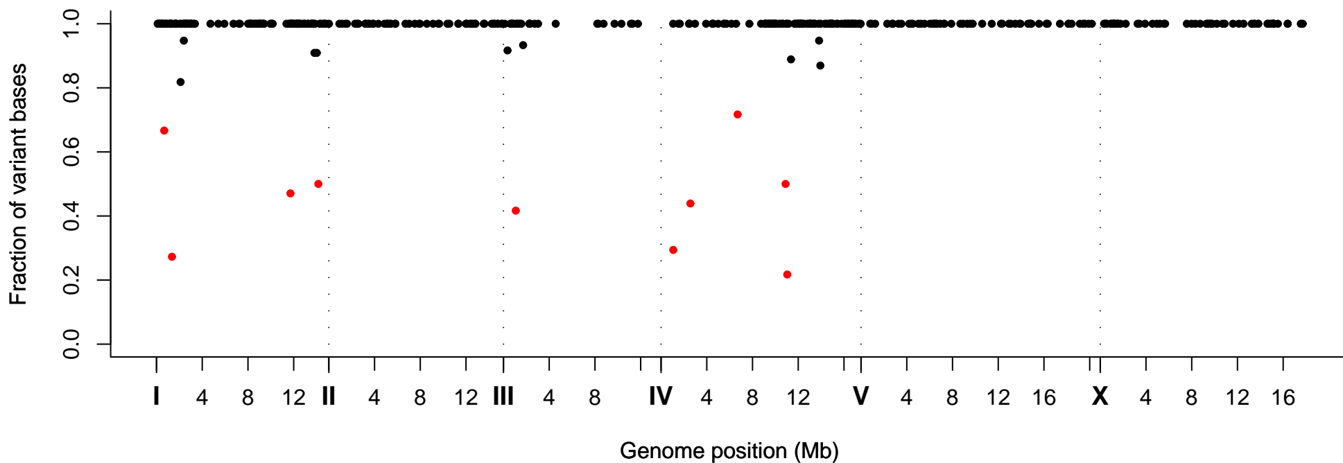
Fraction of Variant Bases at Position, Strain VC40337
