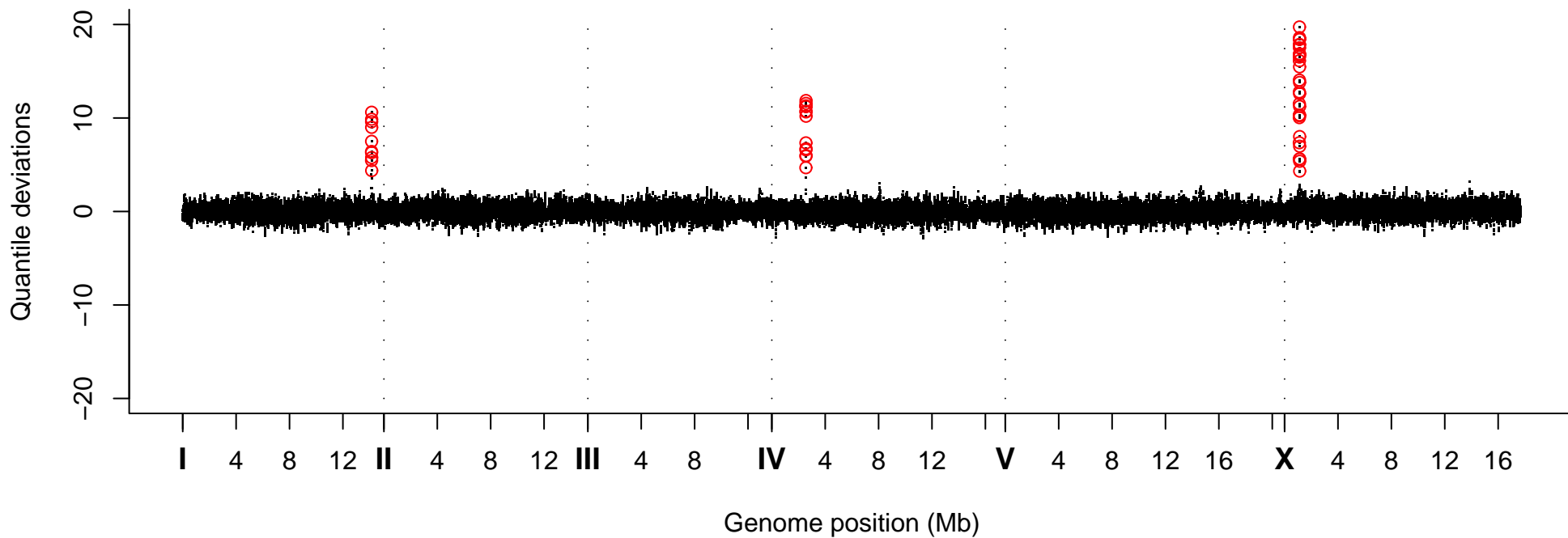
Quantile Deviations, Strain VC40337
