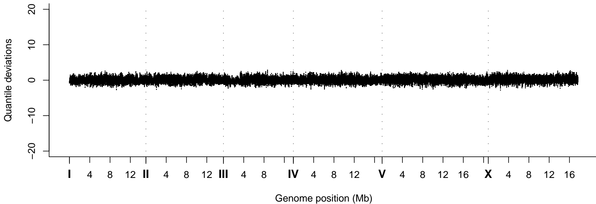
Quantile Deviations, Strain VC40338
