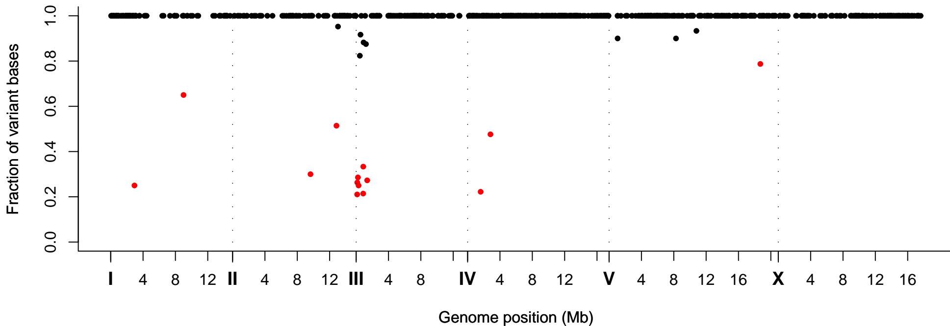
Fraction of Variant Bases at Position, Strain VC40338
