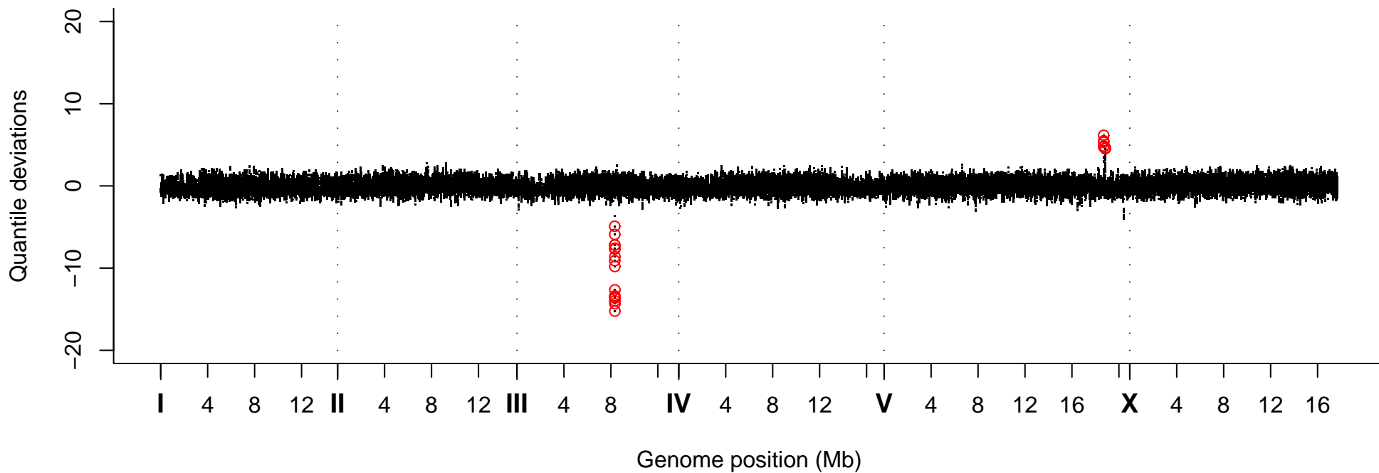
Quantile Deviations, Strain VC40339
