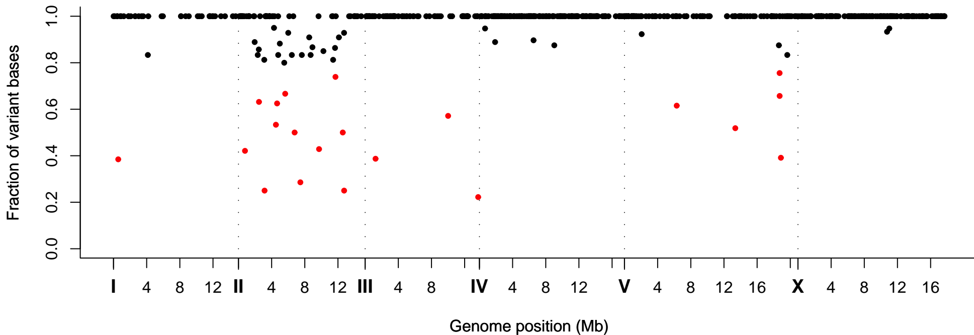
Fraction of Variant Bases at Position, Strain VC40339
