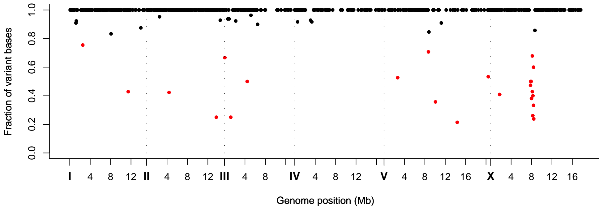
Fraction of Variant Bases at Position, Strain VC40349
