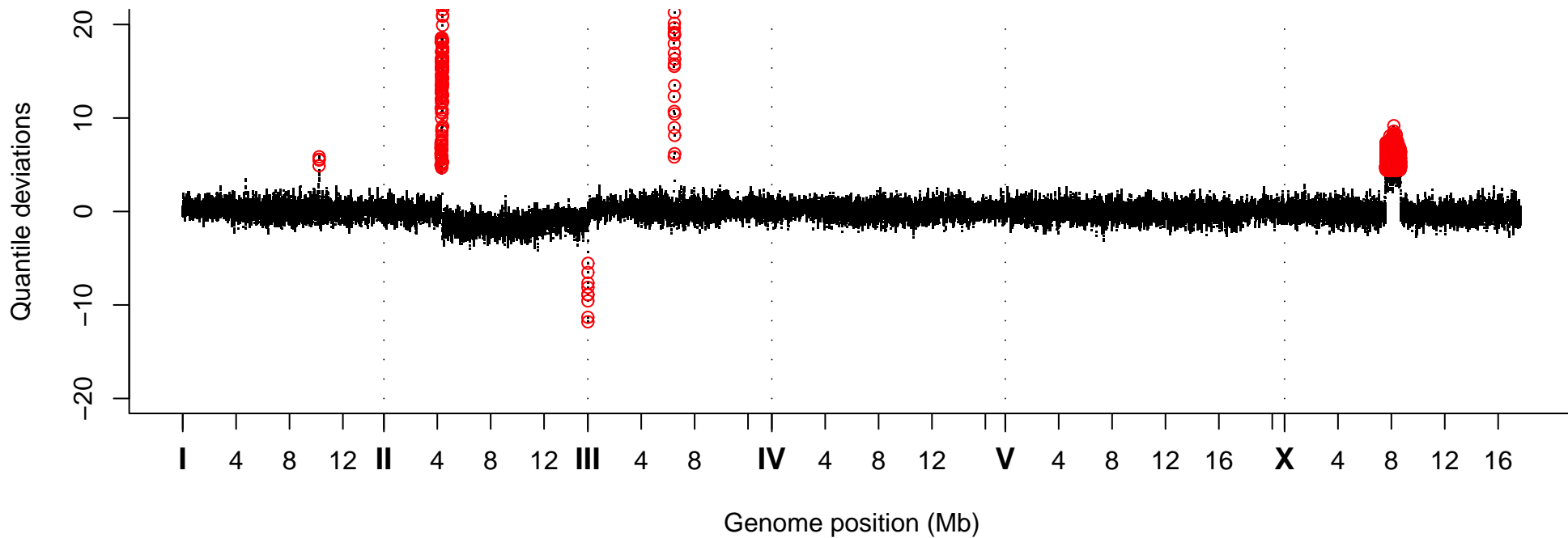
Quantile Deviations, Strain VC40349
