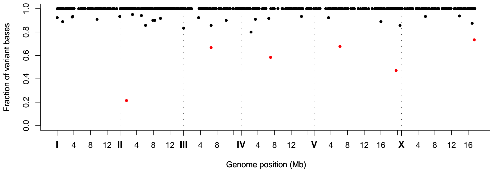
Fraction of Variant Bases at Position, Strain VC40357
