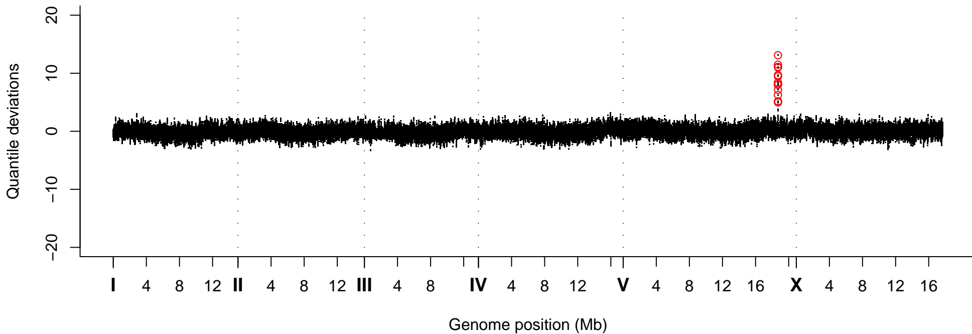
Quantile Deviations, Strain VC40357
