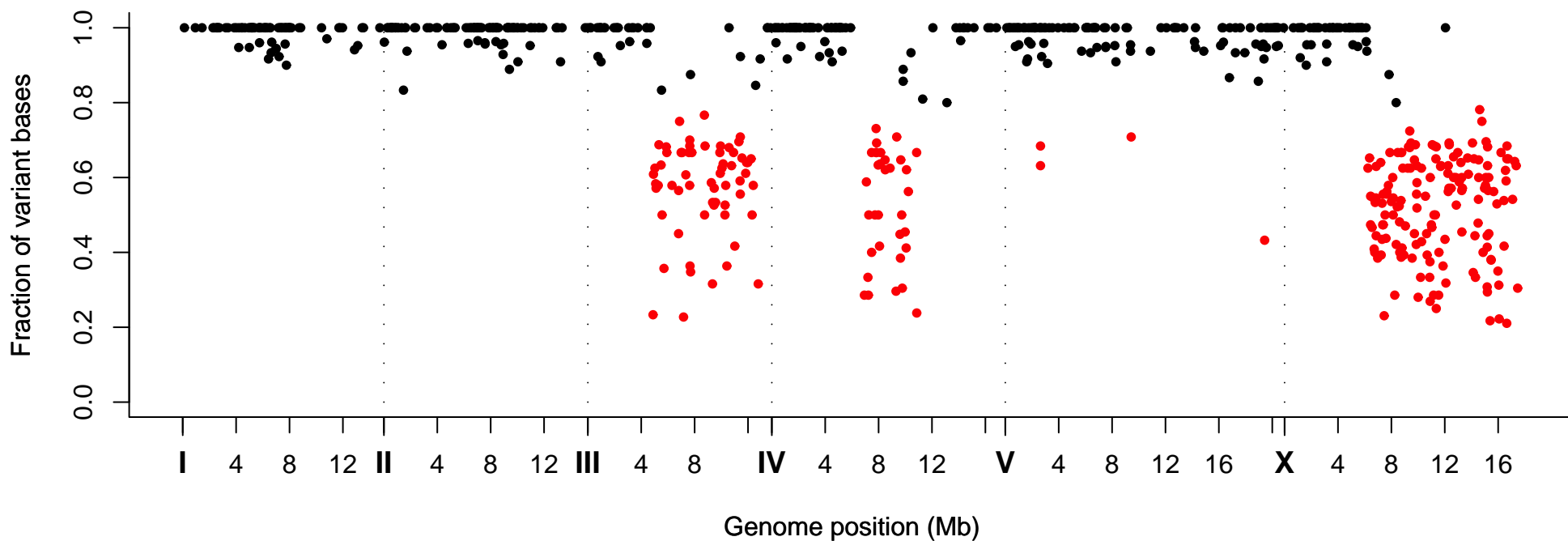
Fraction of Variant Bases at Position, Strain VC40359
