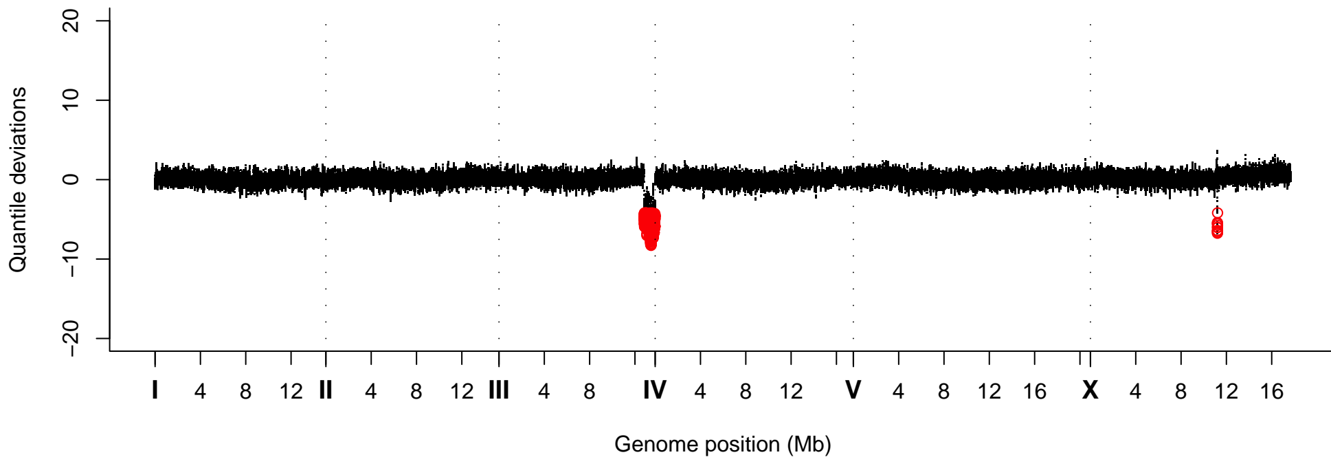
Quantile Deviations, Strain VC40359
