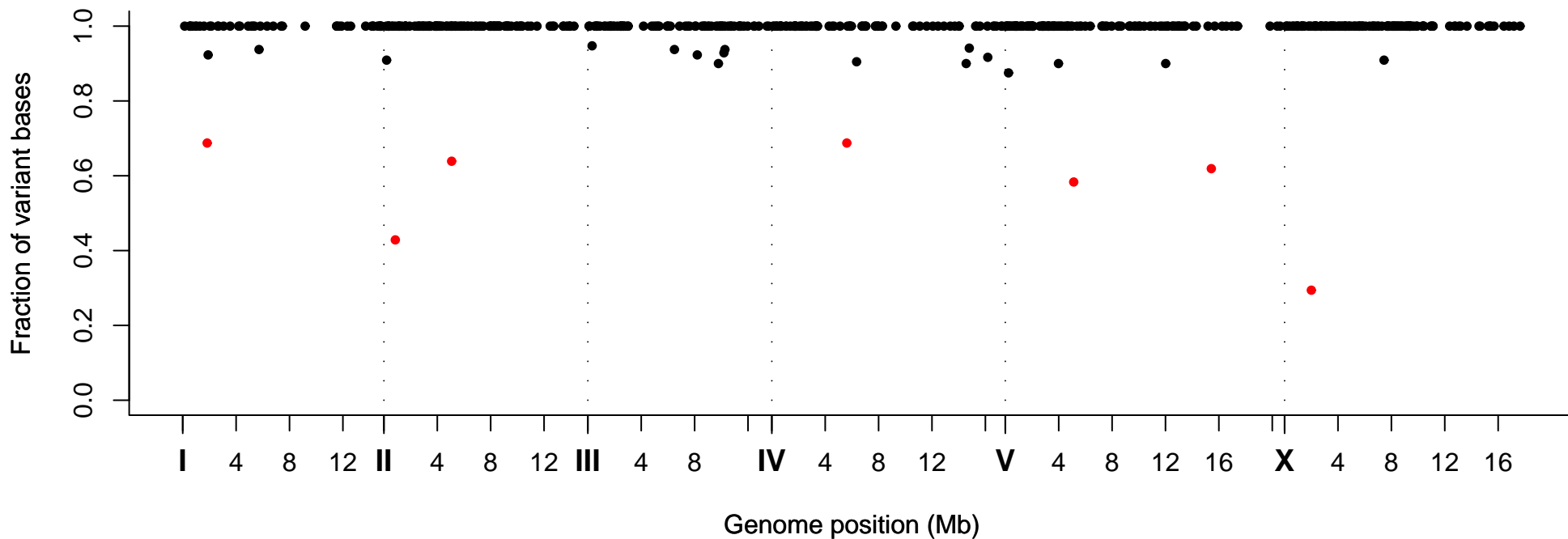
Fraction of Variant Bases at Position, Strain VC40361
