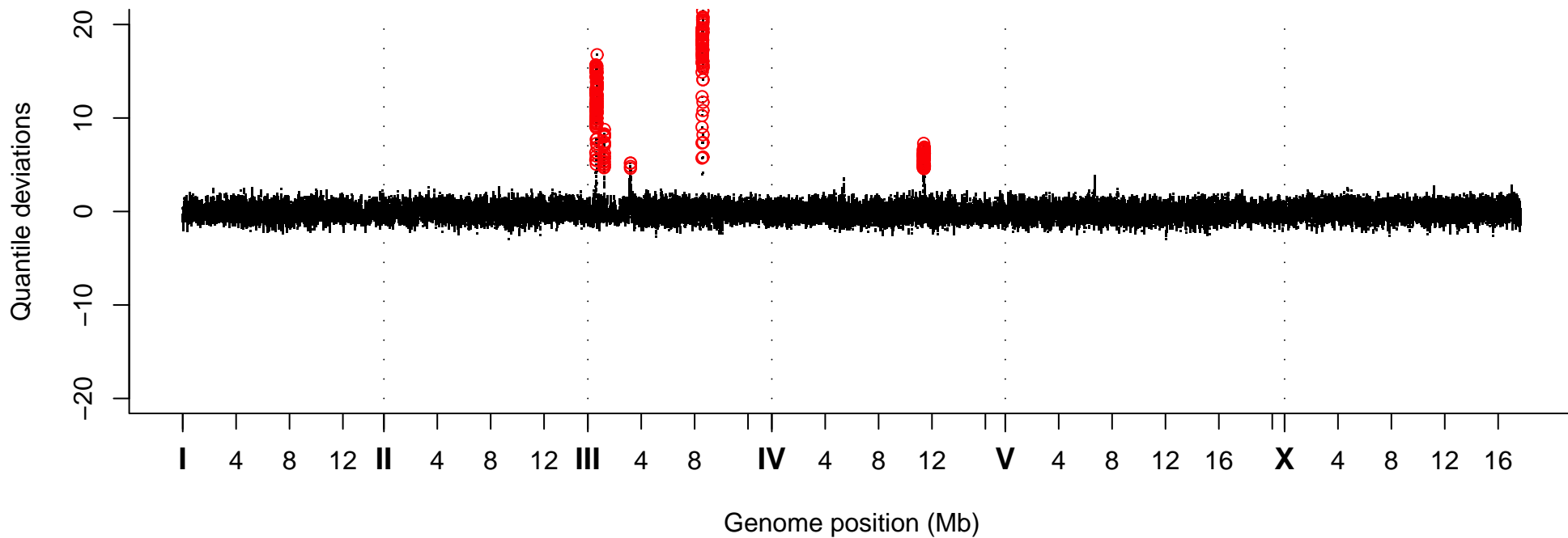
Quantile Deviations, Strain VC40361
