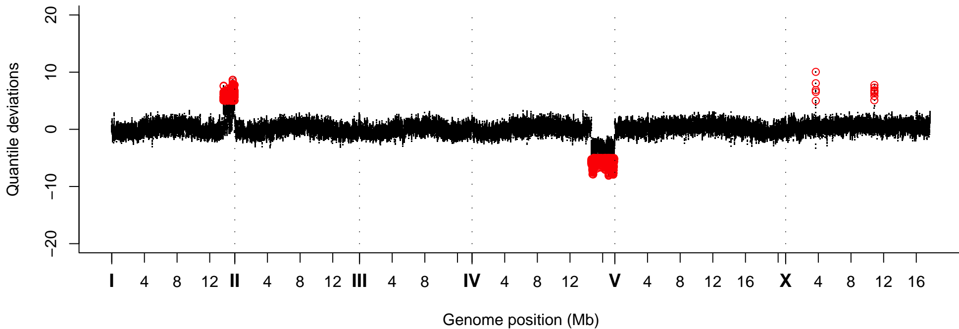
Quantile Deviations, Strain VC40375
