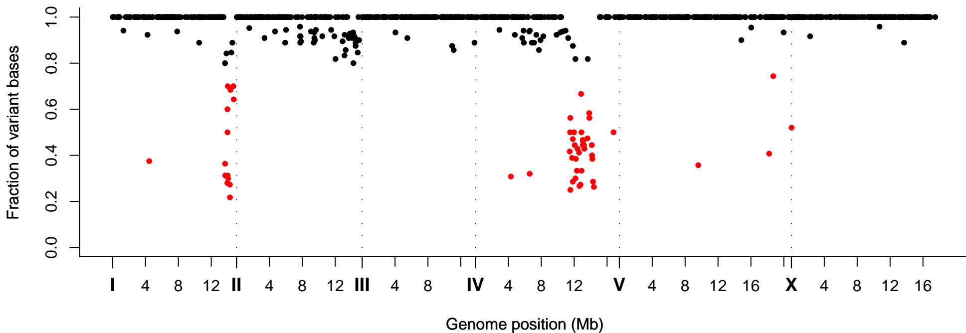
Fraction of Variant Bases at Position, Strain VC40375
