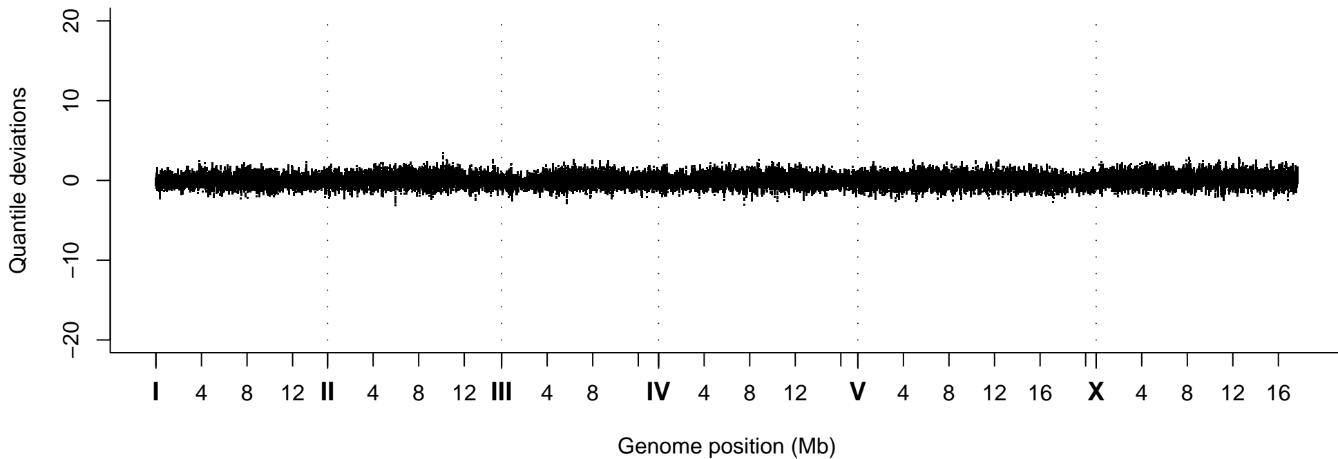
Quantile Deviations, Strain VC40376
