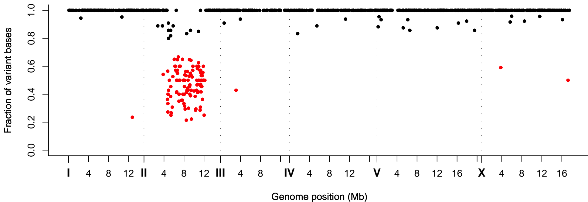
Fraction of Variant Bases at Position, Strain VC40376
