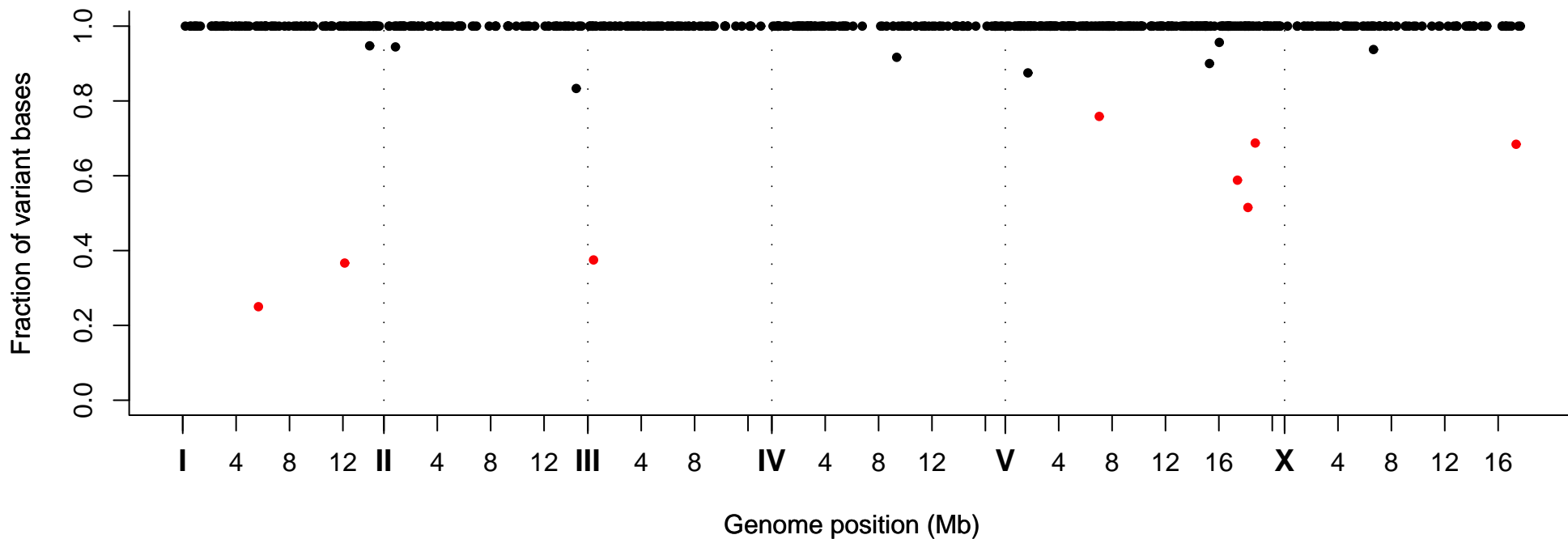
Fraction of Variant Bases at Position, Strain VC40378
