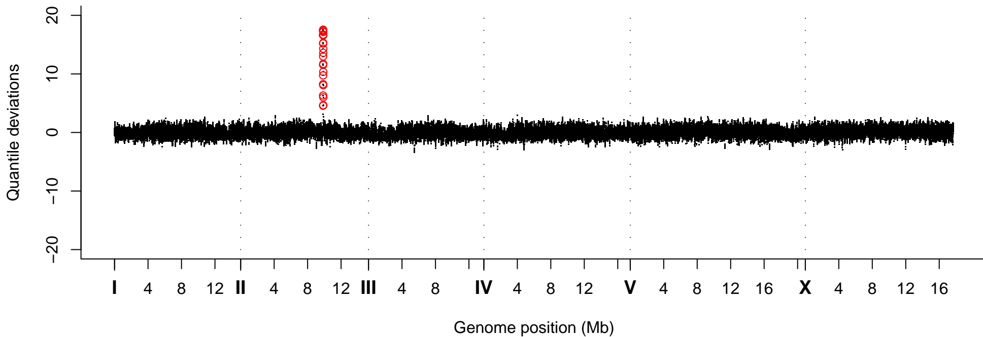
Quantile Deviations, Strain VC40378
