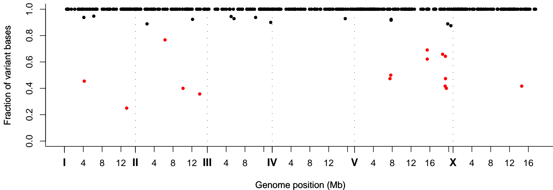
Fraction of Variant Bases at Position, Strain VC40384
