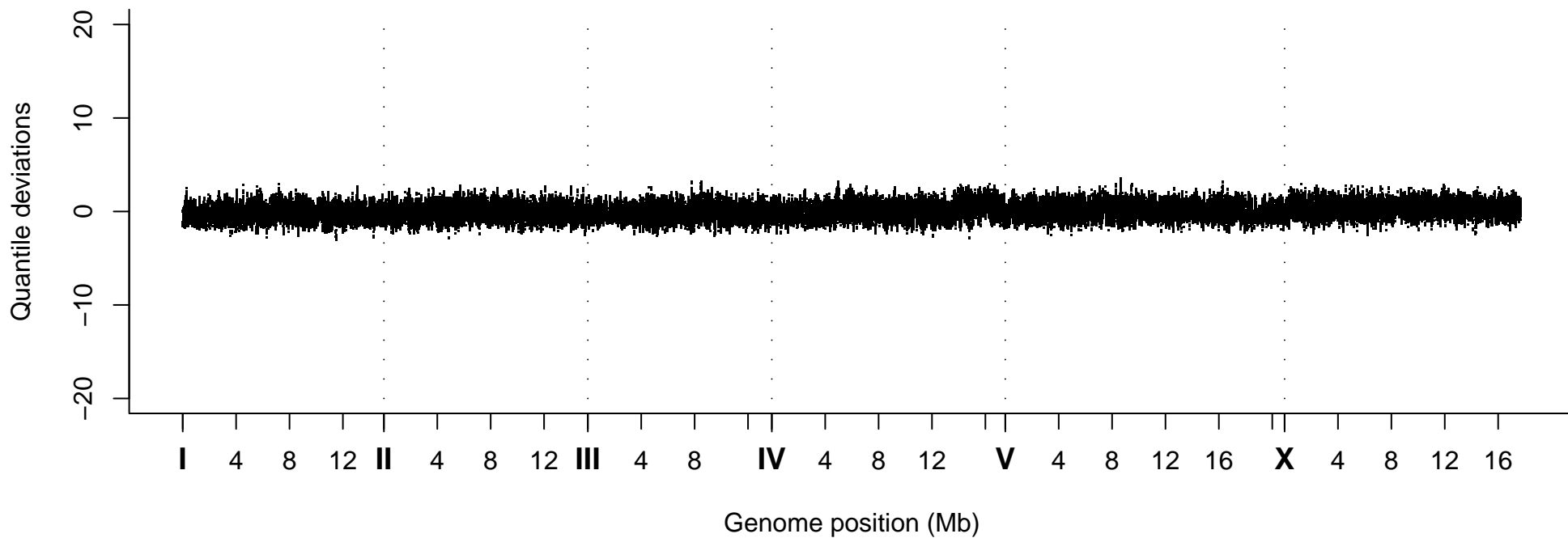
Quantile Deviations, Strain VC40384
