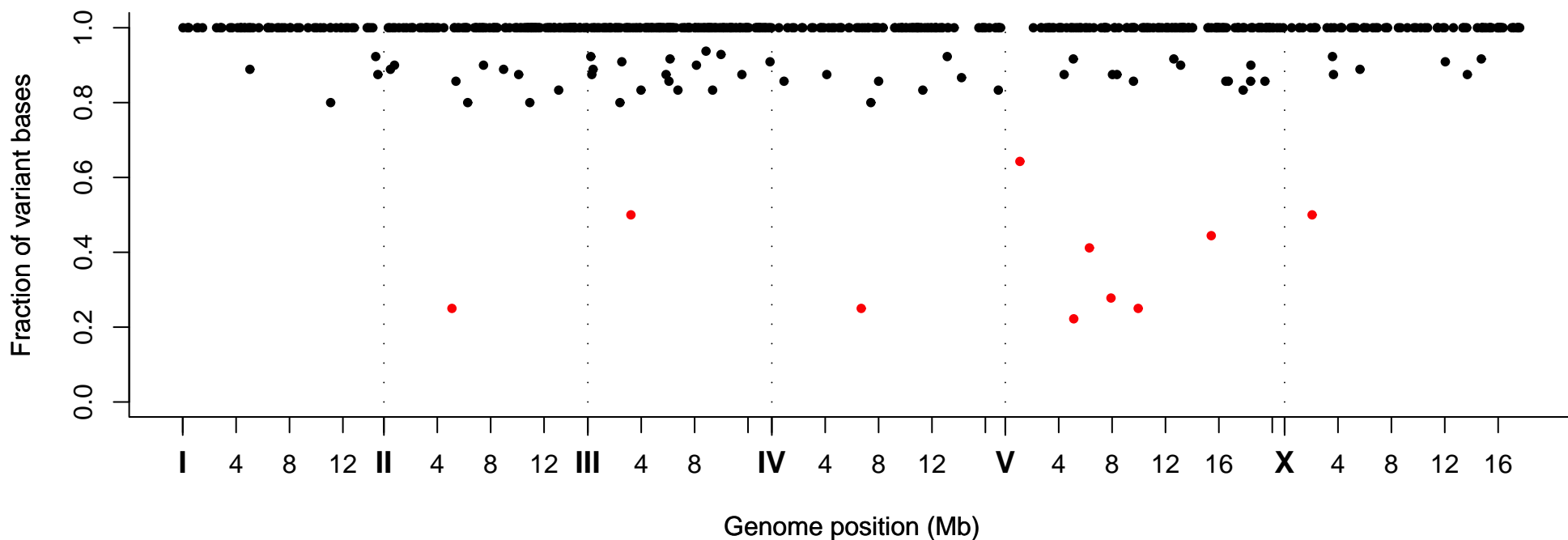
Fraction of Variant Bases at Position, Strain VC40392
