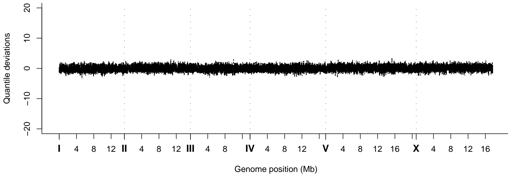
Quantile Deviations, Strain VC40392
