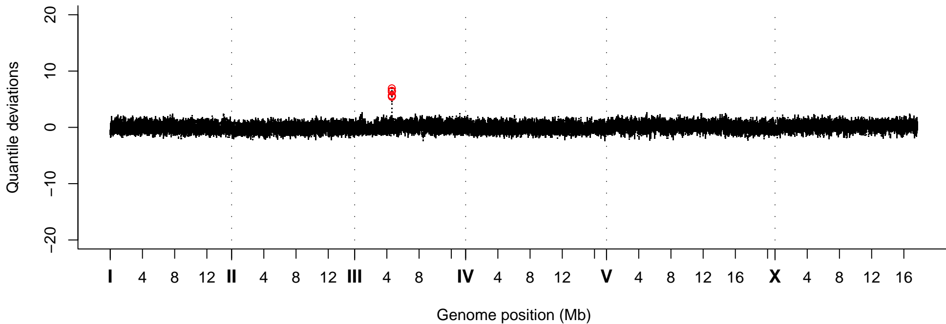
Quantile Deviations, Strain VC40394
