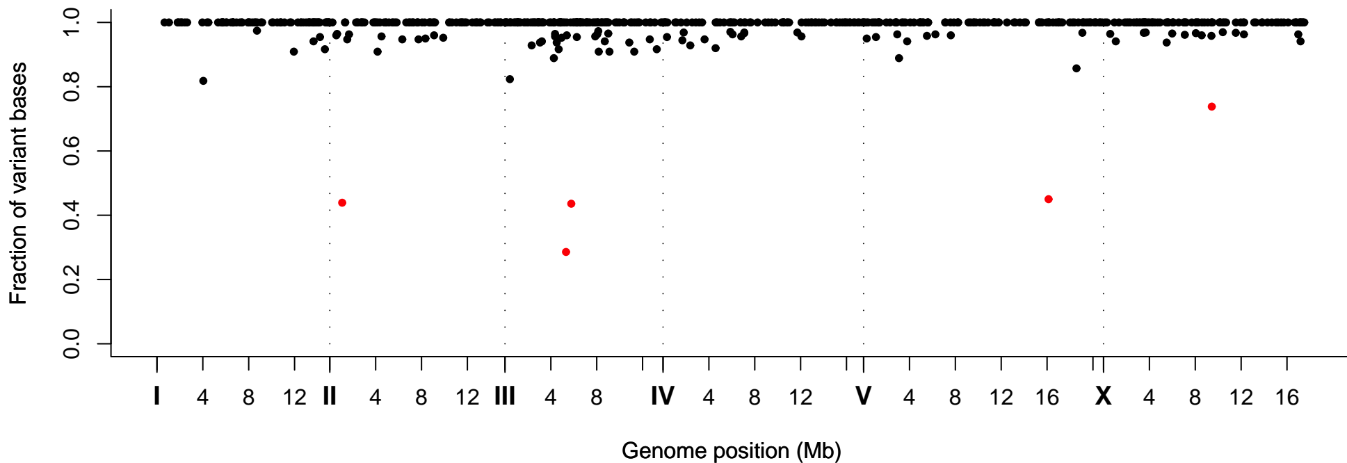
Fraction of Variant Bases at Position, Strain VC40394
