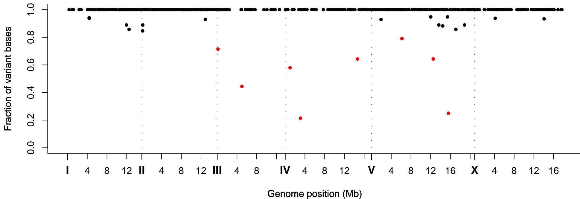
Fraction of Variant Bases at Position, Strain VC40398
