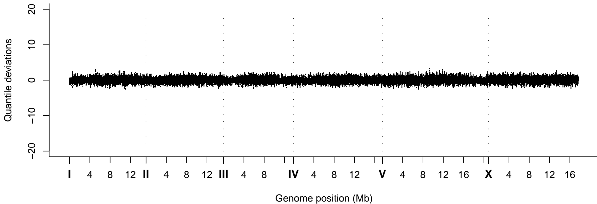
Quantile Deviations, Strain VC40398
