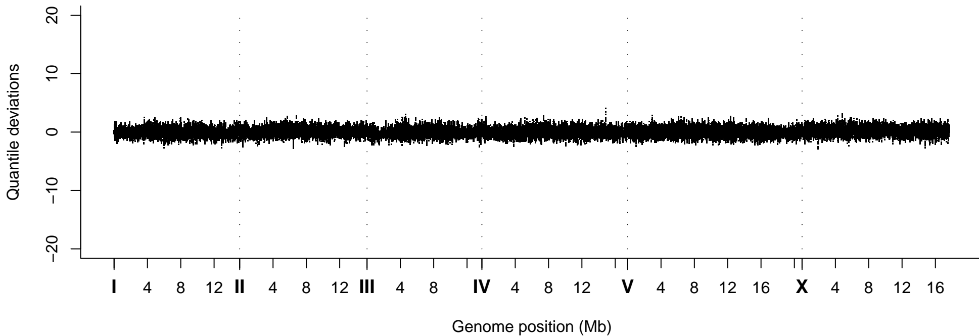
Quantile Deviations, Strain VC40408
