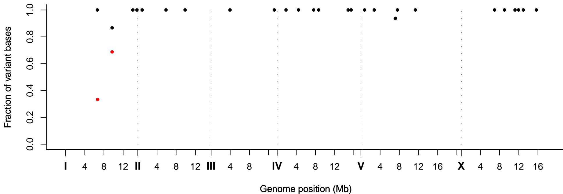
Fraction of Variant Bases at Position, Strain VC40408
