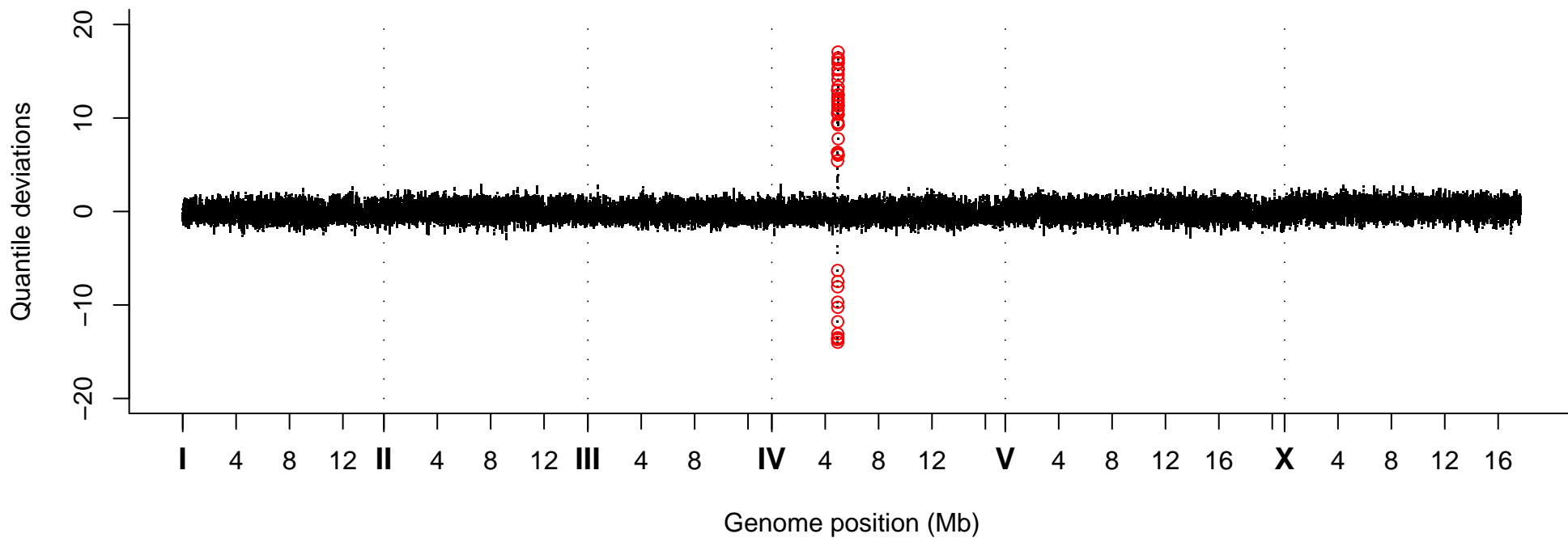
Quantile Deviations, Strain VC40415
