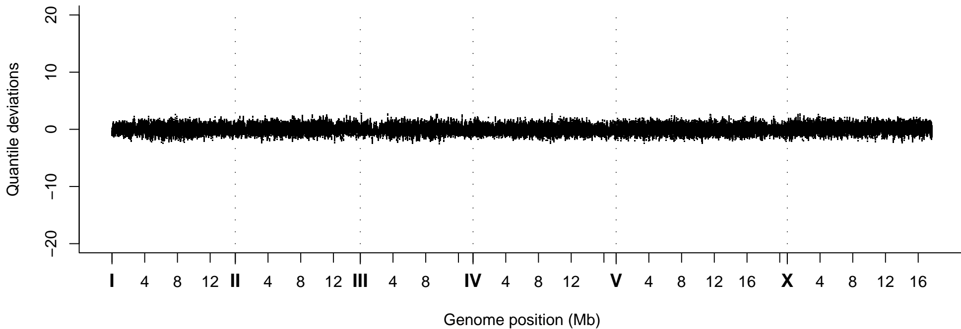
Quantile Deviations, Strain VC40418
