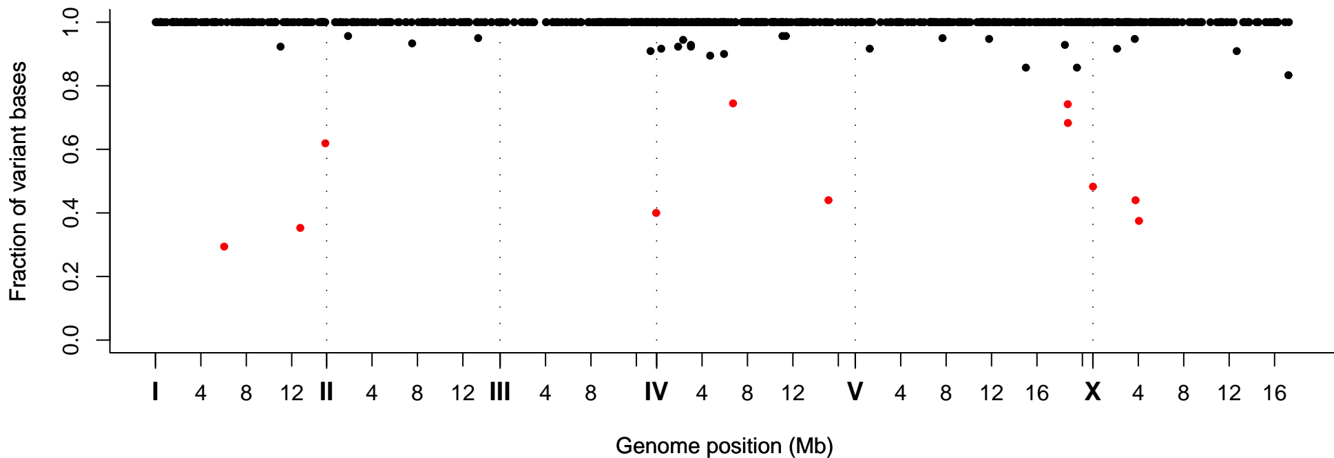
Fraction of Variant Bases at Position, Strain VC40418
