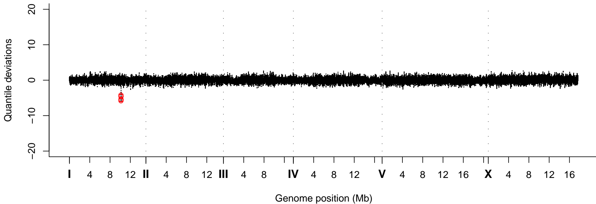
Quantile Deviations, Strain VC40419
