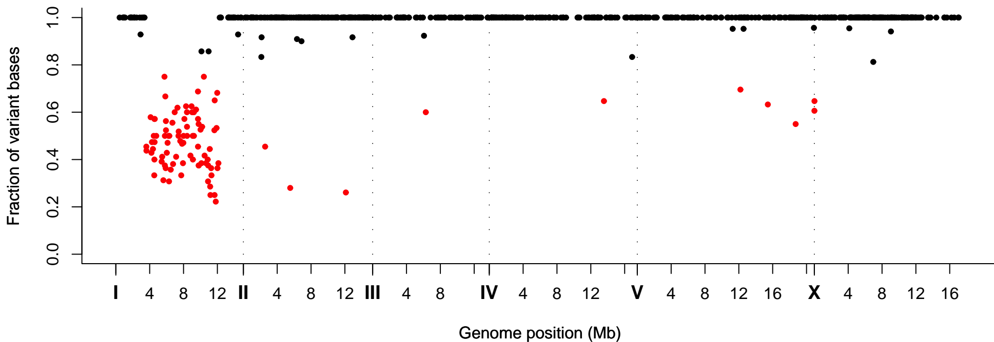
Fraction of Variant Bases at Position, Strain VC40419
