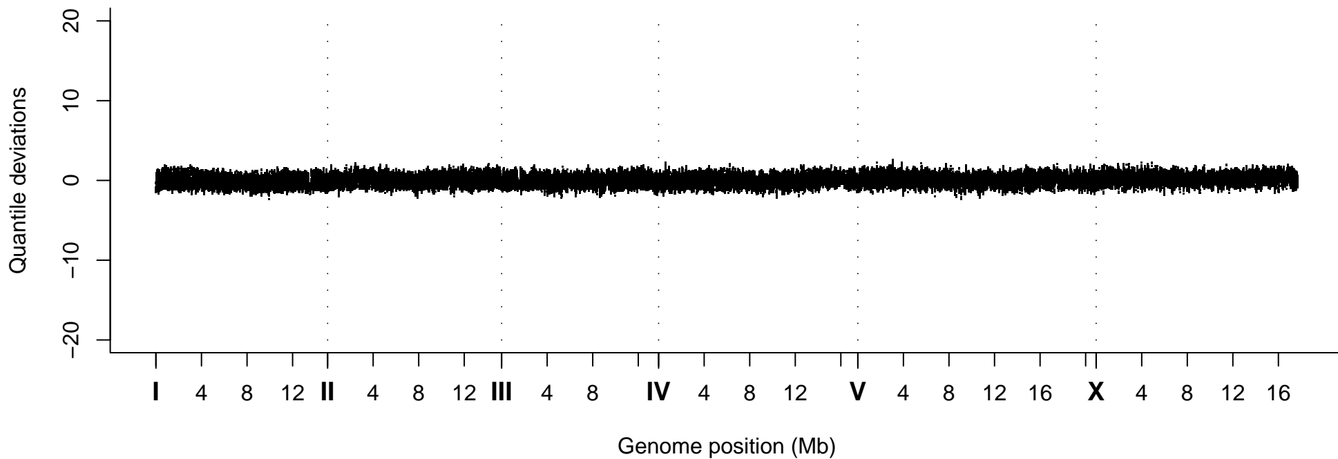
Quantile Deviations, Strain VC40422
