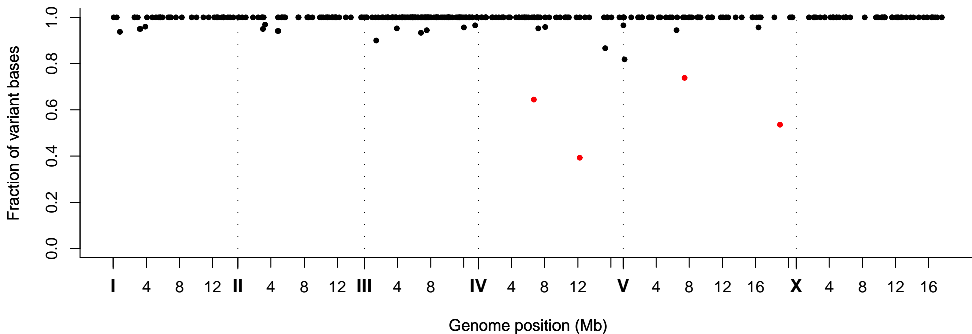
Fraction of Variant Bases at Position, Strain VC40422
