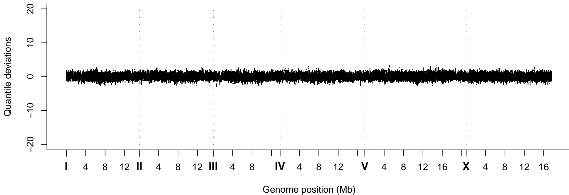
Quantile Deviations, Strain VC40424
