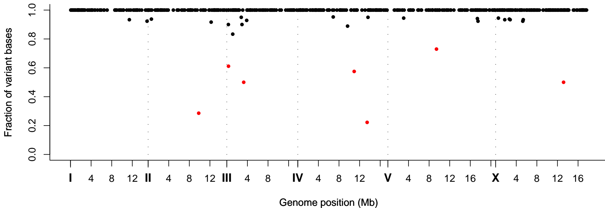
Fraction of Variant Bases at Position, Strain VC40424
