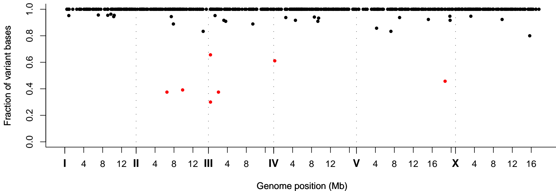
Fraction of Variant Bases at Position, Strain VC40427
