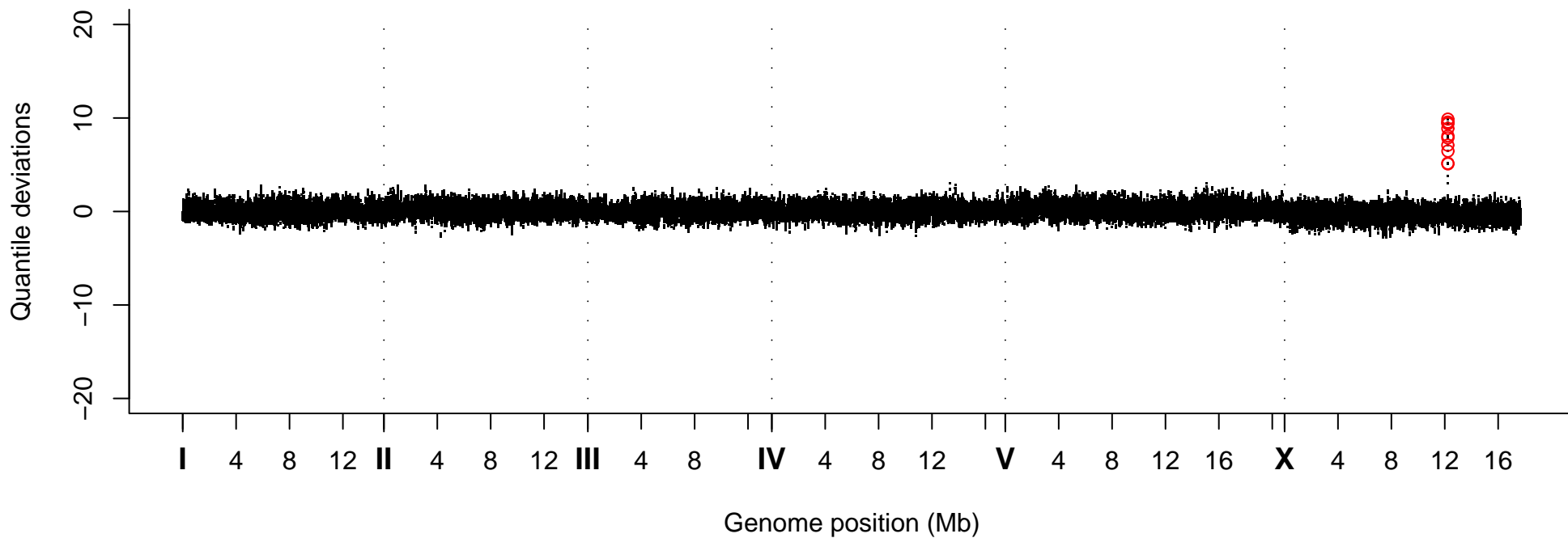
Quantile Deviations, Strain VC40427
