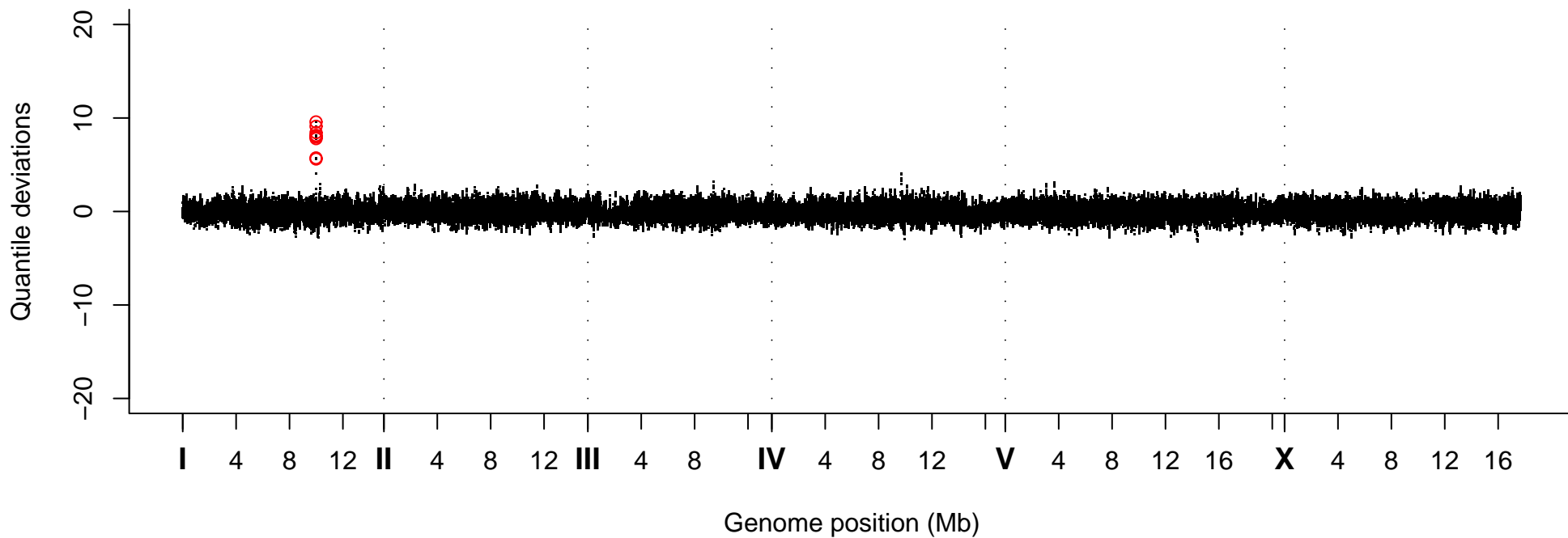
Quantile Deviations, Strain VC40428
