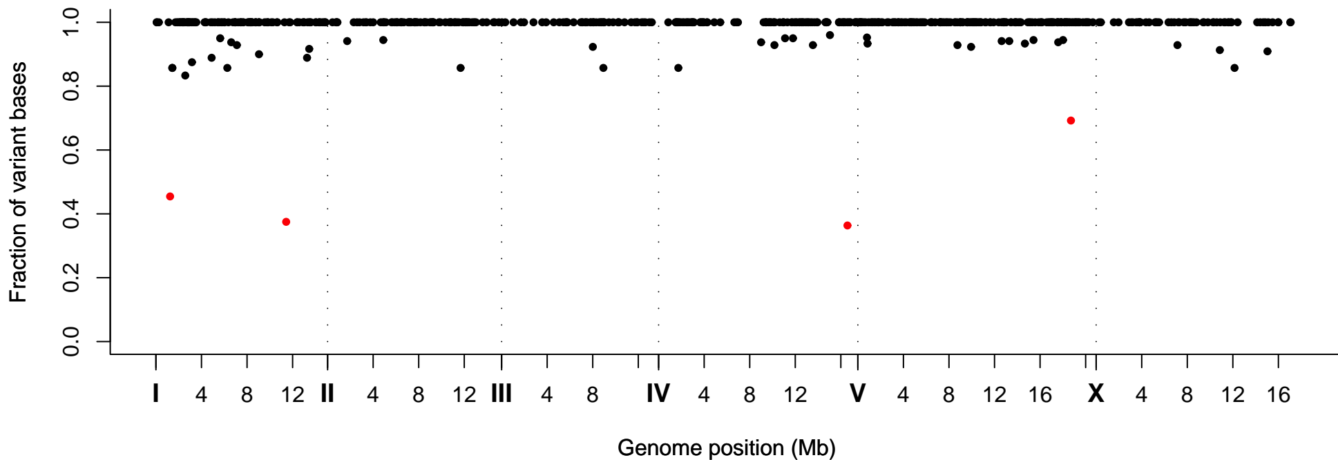
Fraction of Variant Bases at Position, Strain VC40428
