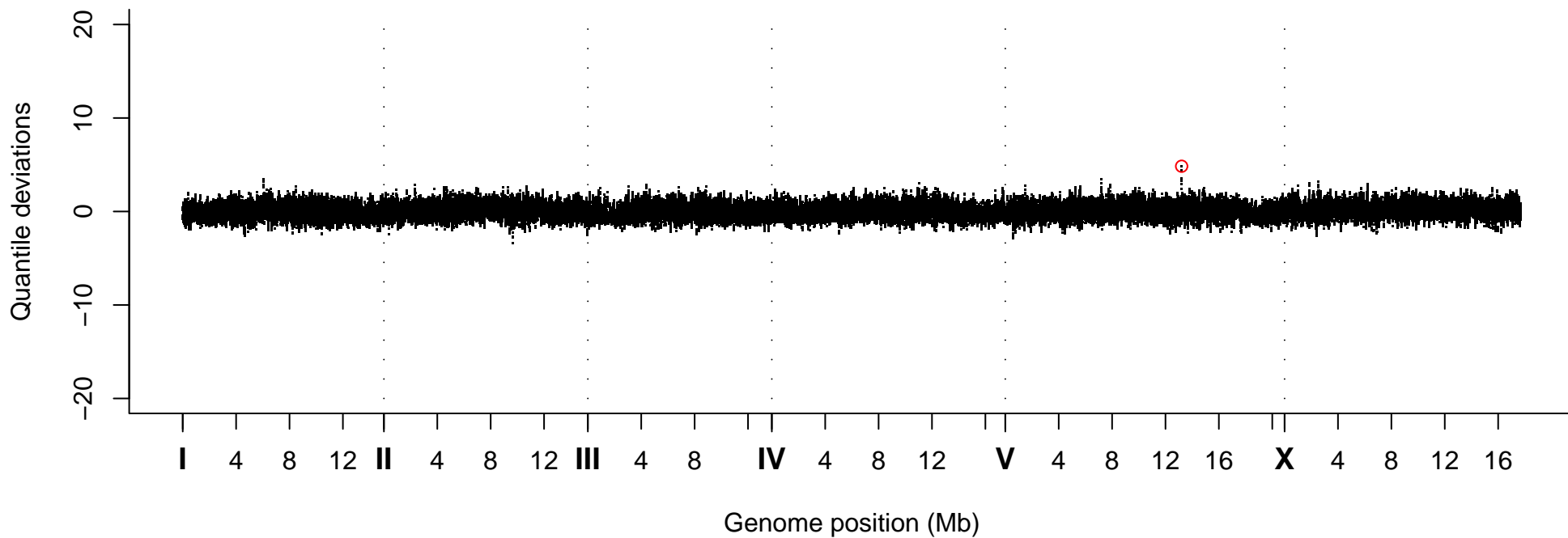
Quantile Deviations, Strain VC40437
