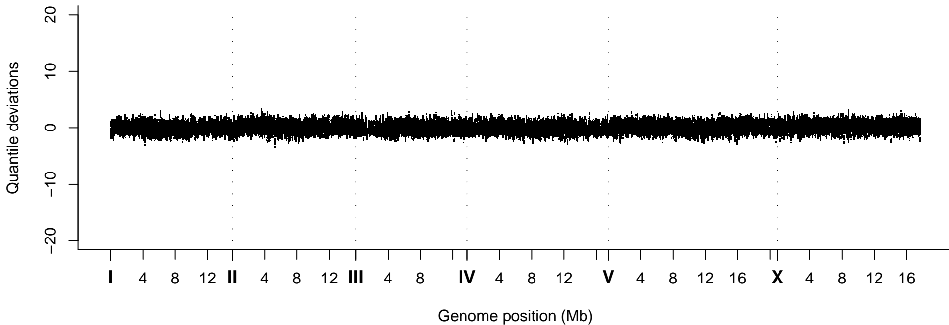
Quantile Deviations, Strain VC40448
