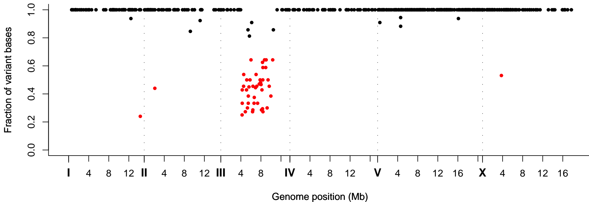
Fraction of Variant Bases at Position, Strain VC40448
